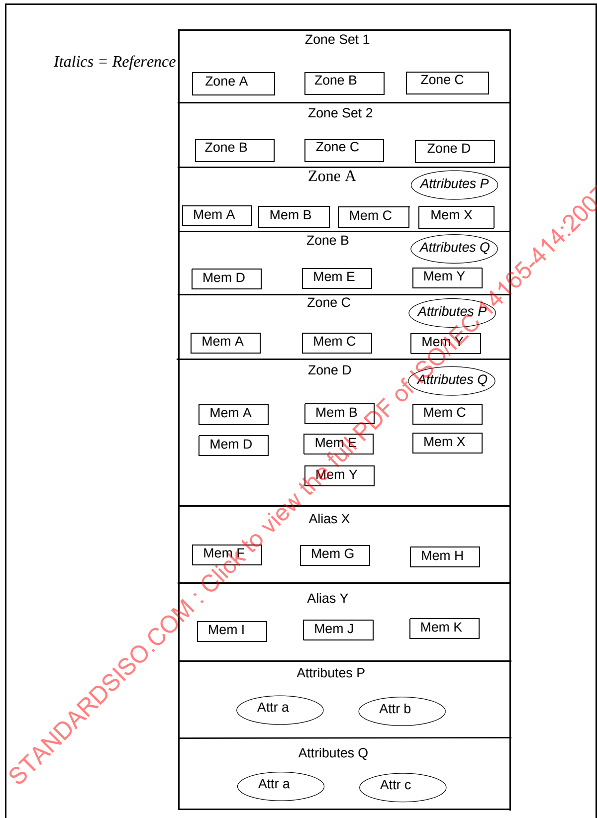
Figure 13 – Logical Structure of the Zone Set Database
