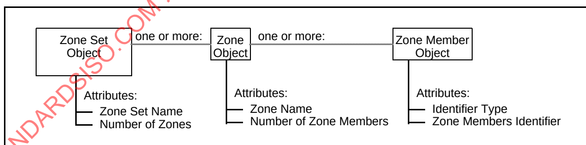
Figure 12 – Zone Set, Zone and Zone Member attributes
