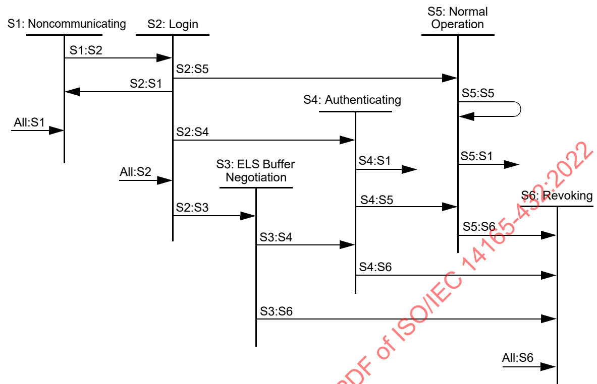
Figure 30 – NFA State Machine
