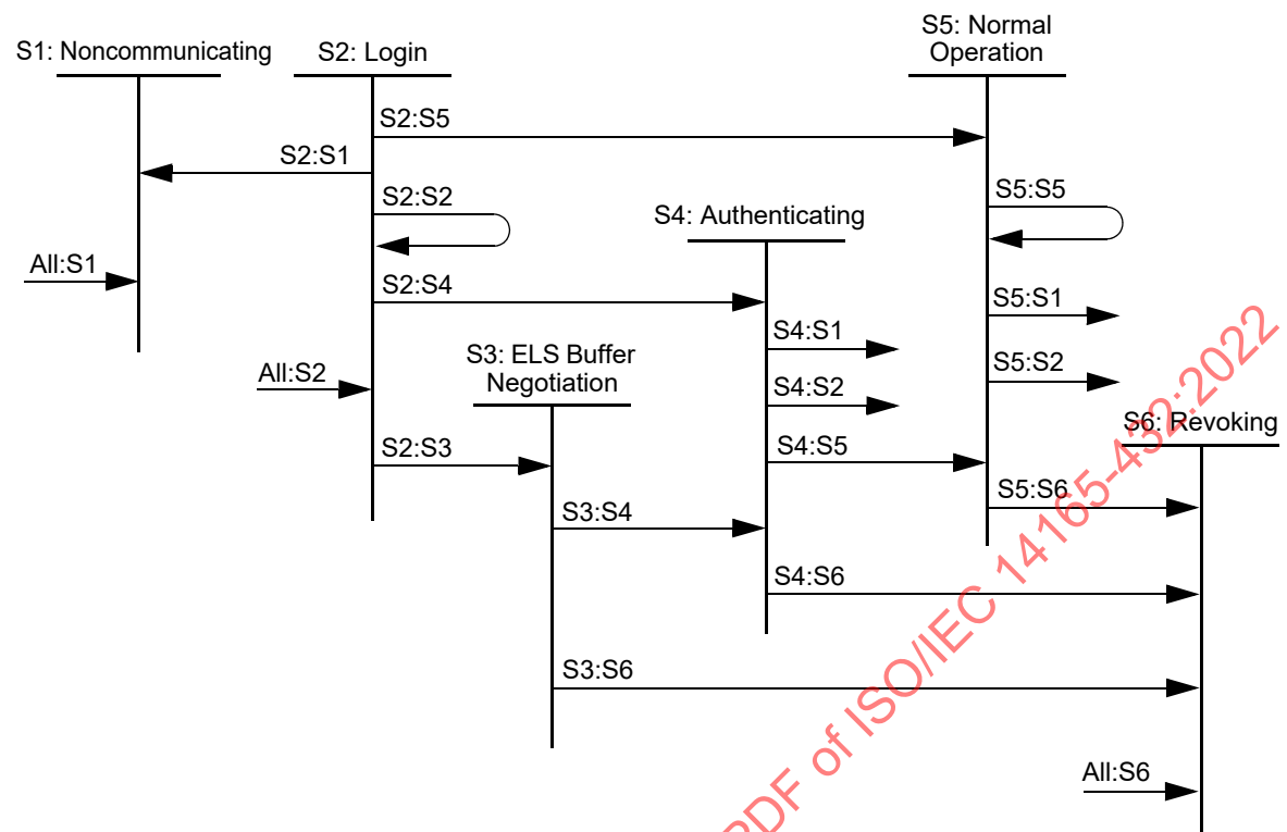
Figure 31 – FNA State Machine
