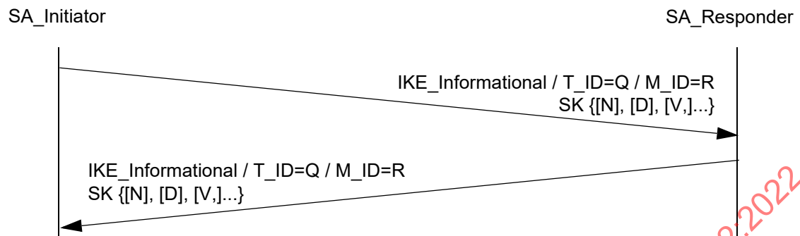
Figure 23 – An IKE_Informational exchange.
