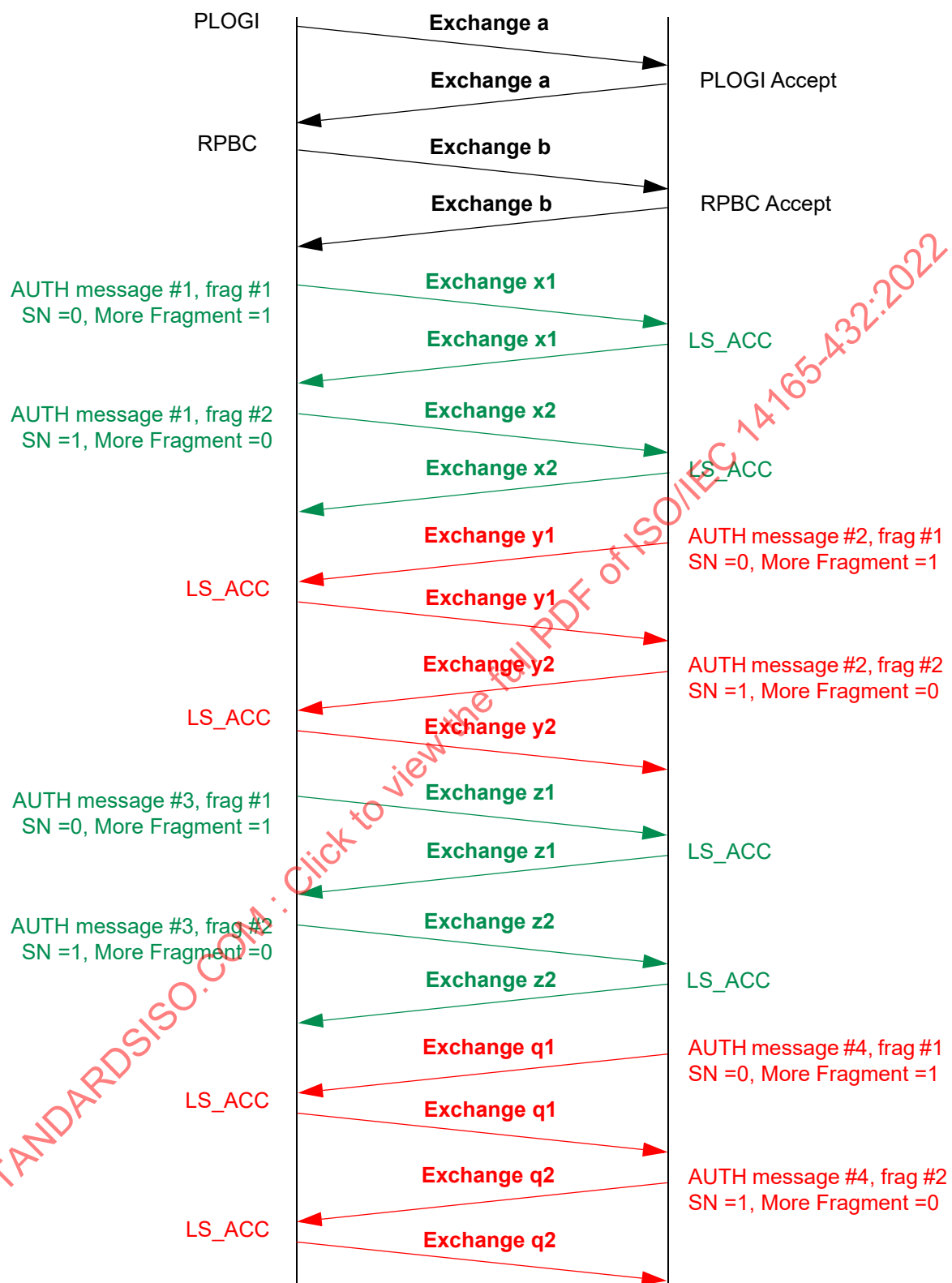
Figure 18 – FC-2 Authentication Mapping with AUTH_ELS Fragmentation Example
