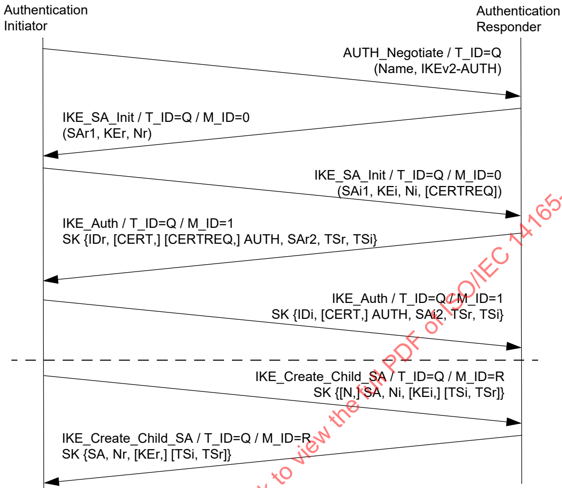
Figure 25 – An IKEv2-AUTH Transaction.
