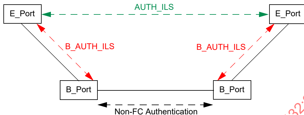
Figure 13 – Usage of B_AUTH_ILS
