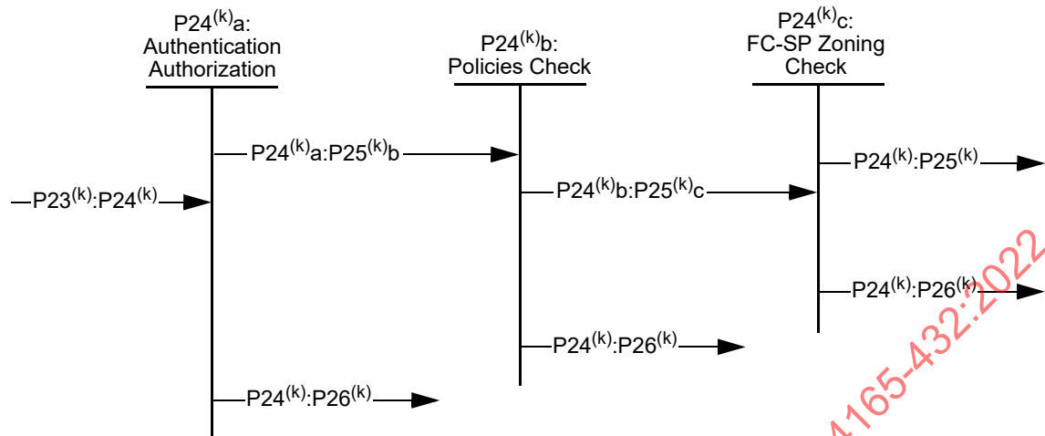
Figure 34 – State P24^{(k)} :Security Checks
