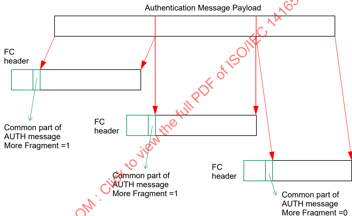
Figure 16 – AUTH_ELS Fragmentation Process
