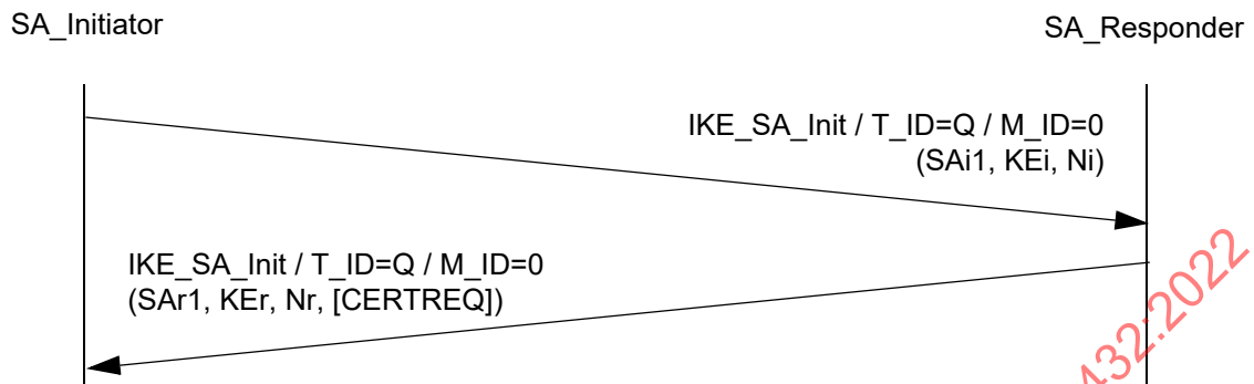
Figure 20 – An IKE_SA_Init exchange.
