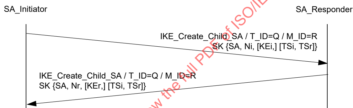
Figure 22 – An IKE_Create_Child_SA exchange.
