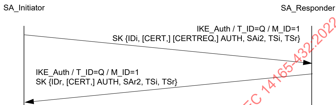
Figure 21 – An IKE_Auth exchange.
