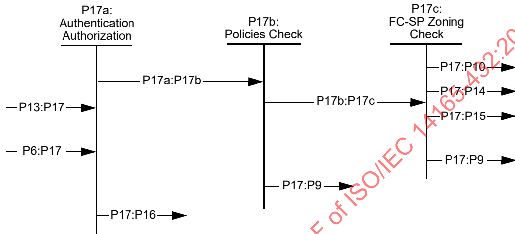
Figure 33 – State P17: Security Checks
