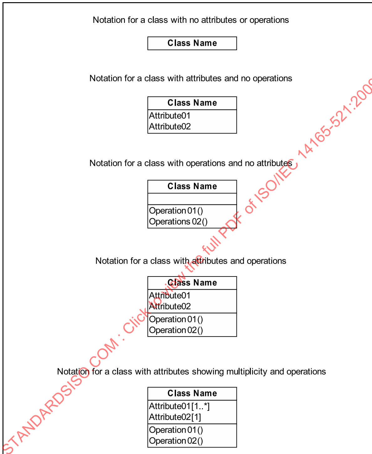
Figure 1 – Class diagram conventions
