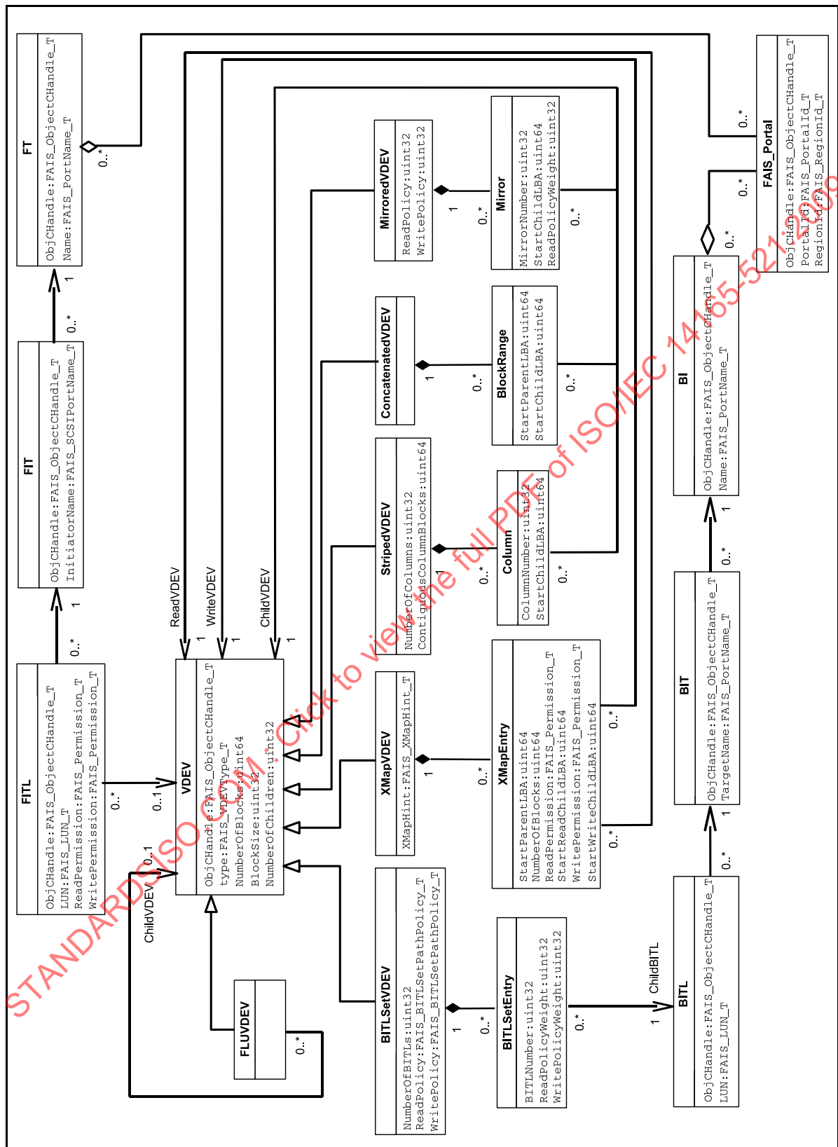
Figure 6 – Object model
