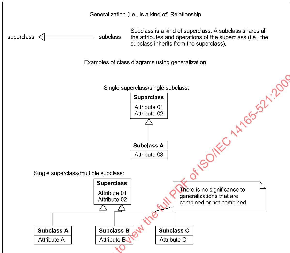
Figure 4 – Notation for generalization relationships for class diagrams
