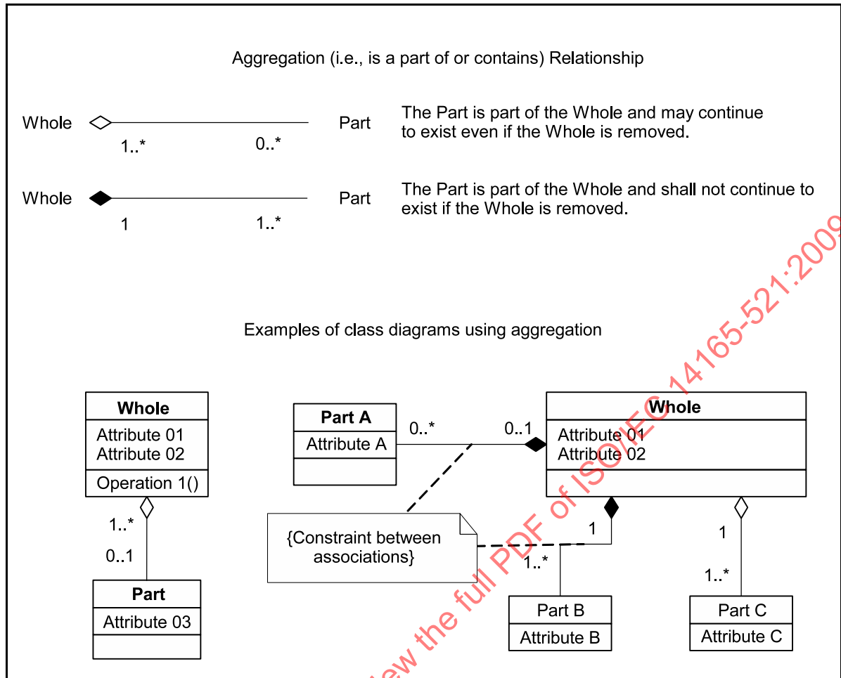
Figure 3 – Notation for aggregation relationships for class diagrams
