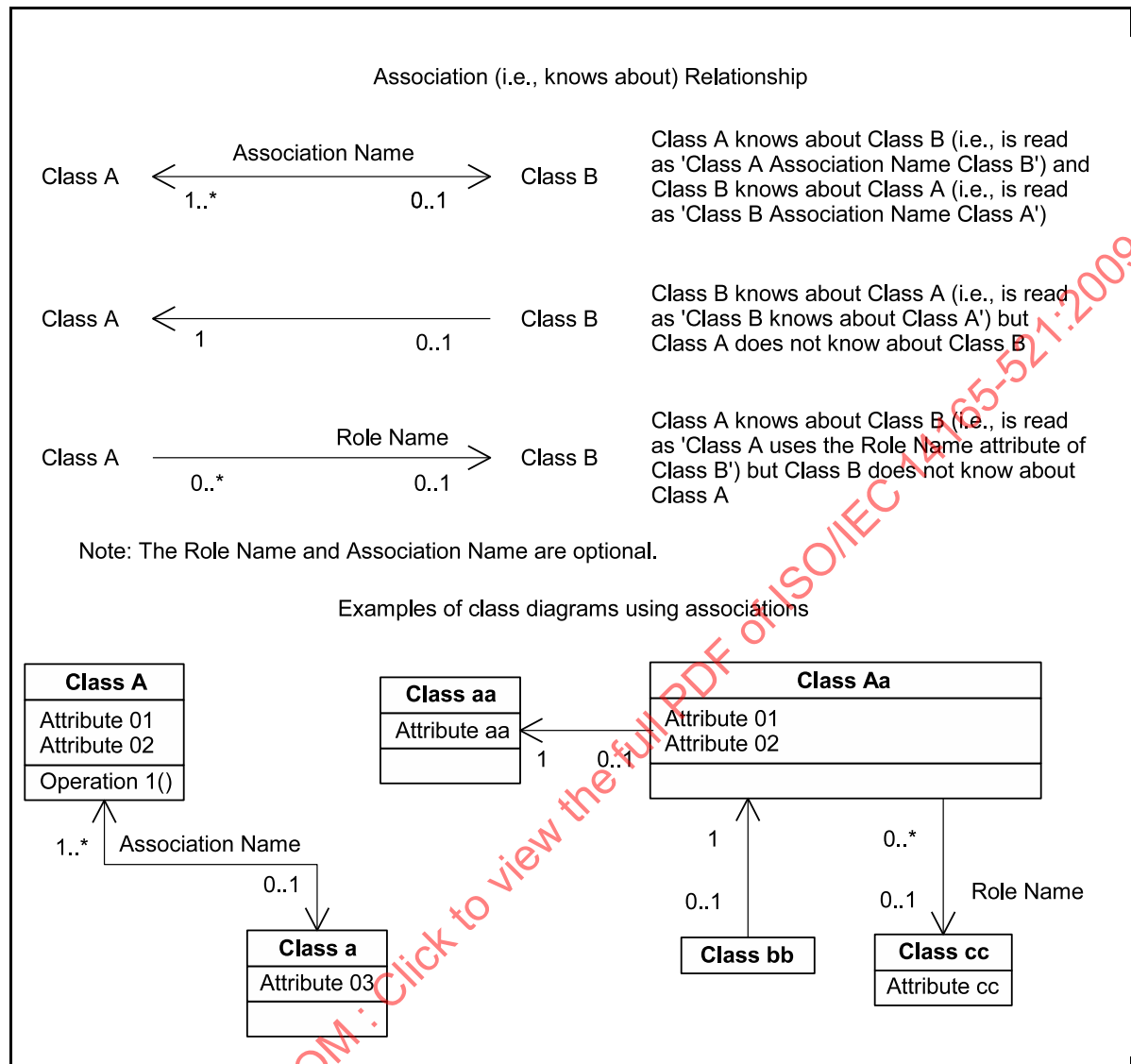
Figure 2 – Notation for association relationships for class diagrams
