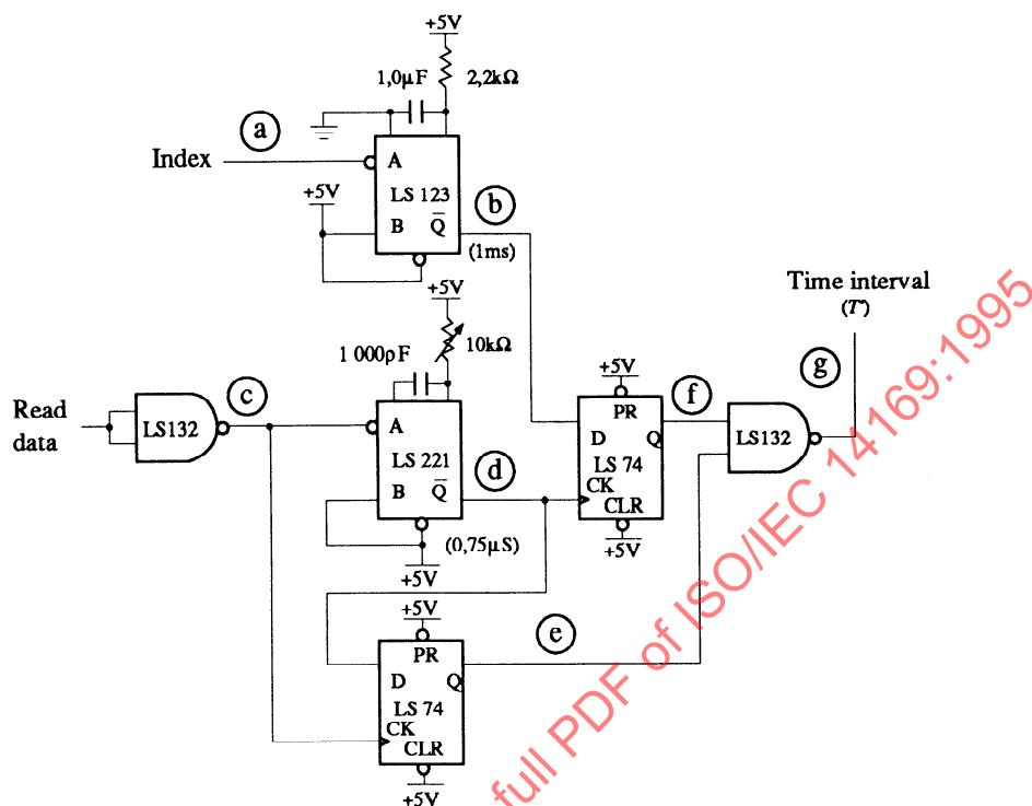
Figure F.1 - Measurement Circuit
