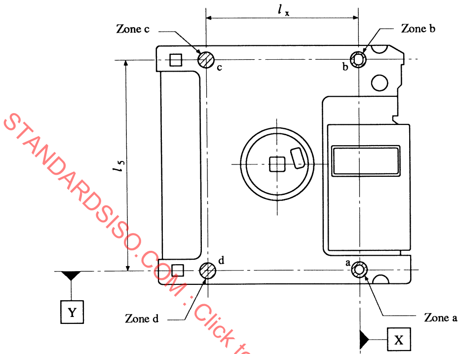
Figure C.1 - Location of the reference zones
