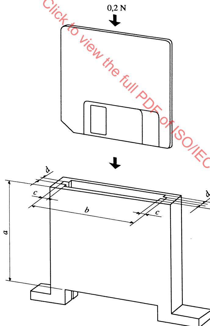
Figure A.1 - Test gauge
