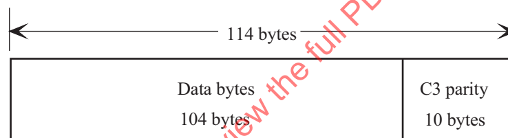
Figure 6 - C3 Error correction code block
