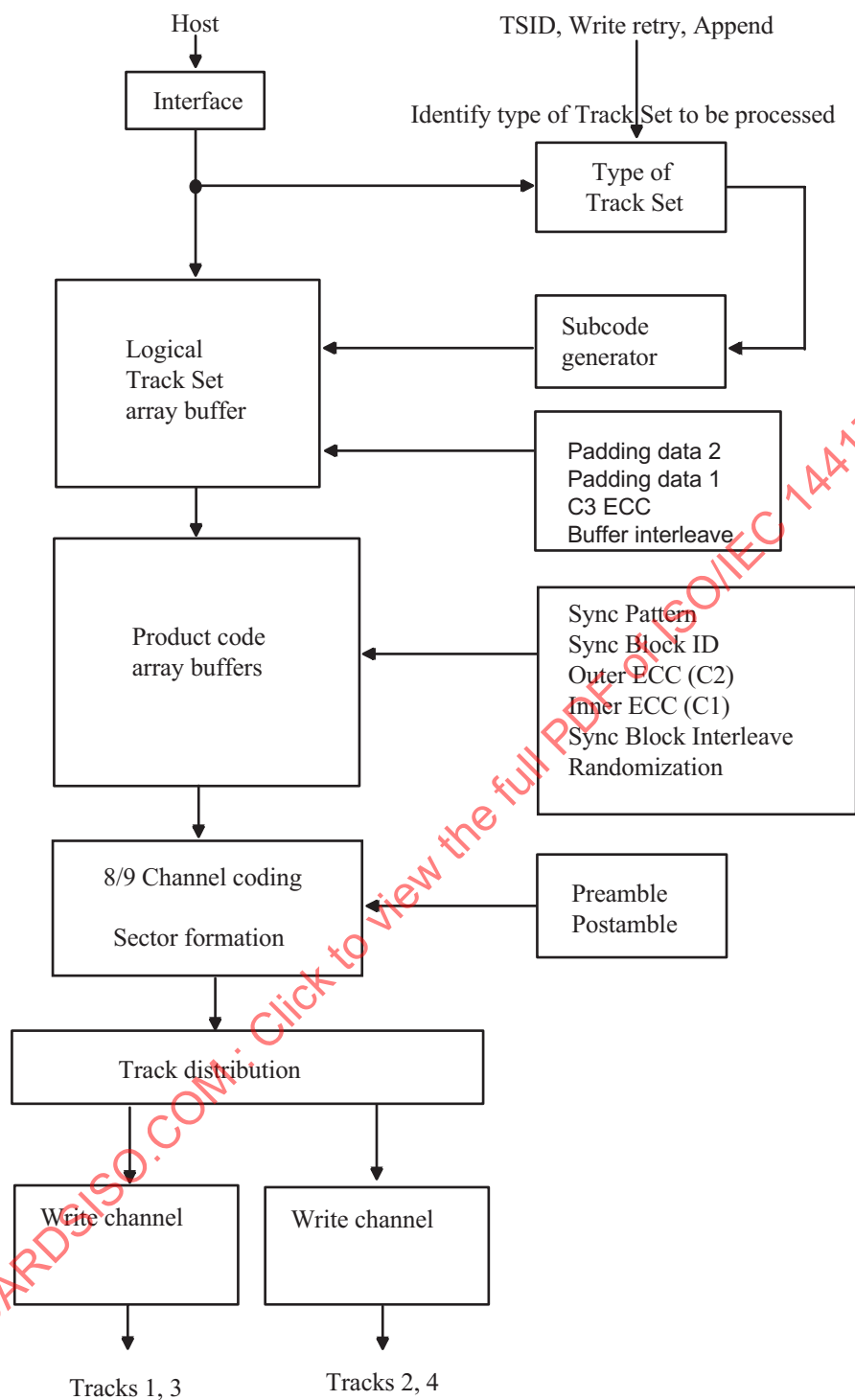
Figure 4 - Dataflow of record information processing
