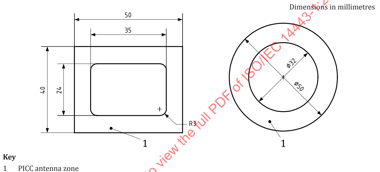
Figure A.3 — Location of the antenna of the “Class 3” PICC
