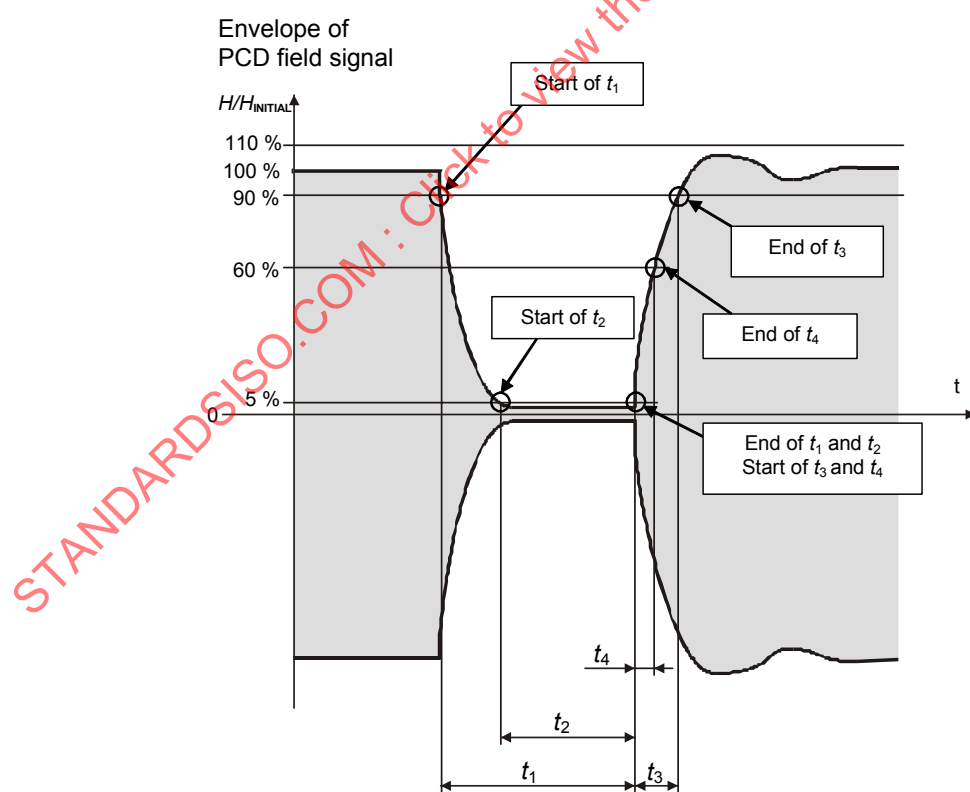
Figure 3 — PauseA for a bit rate of fc/128
