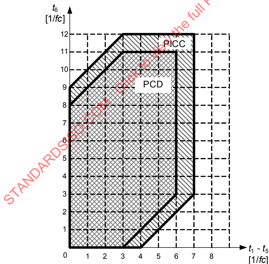
Figure 7 — PauseA timing parameters for a bit rate of fc/64
