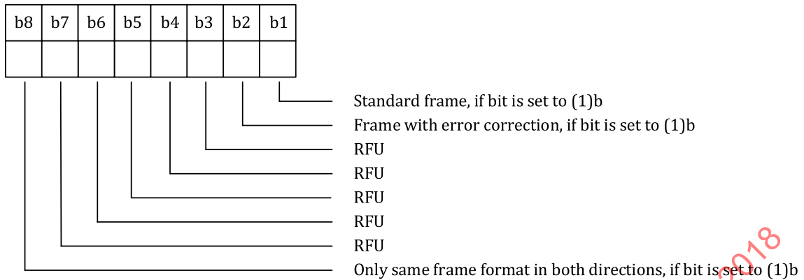
Figure 37 — Frame formats
