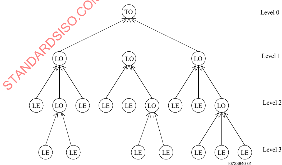
Figure 4 – An ECTP Control Tree
