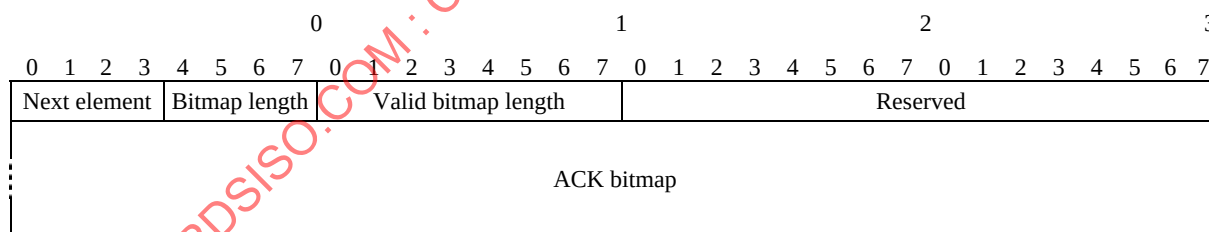
Figure 11 – Acknowledgement extension element
