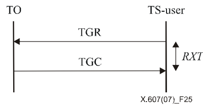
Figure 25 – Token Get procedure
