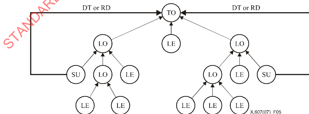
Figure 5 – Backward data channels in ECTP-3
