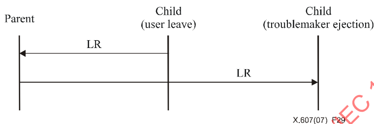
Figure 29 – User leave and troublemaker ejection procedures
