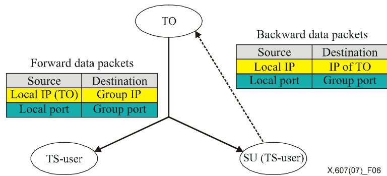
Figure 6 – Data channel addressing in ECTP-3
