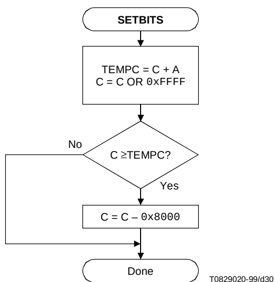
Figure E.12 – Setting the final bits in the C register
