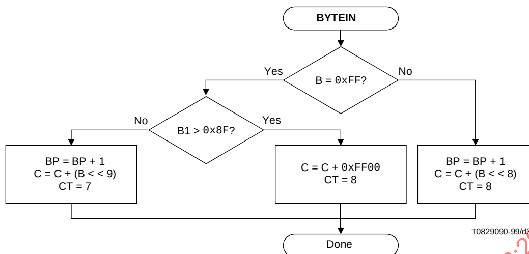
Figure E.19 – BYTEIN procedure for decoder
