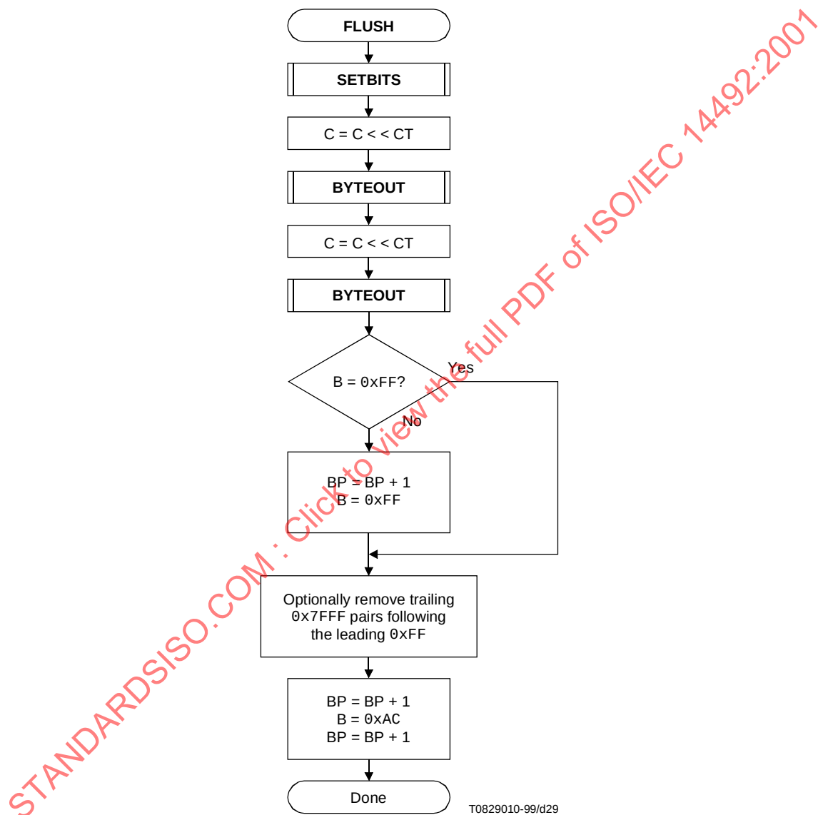
Figure E.11 – FLUSH procedure
