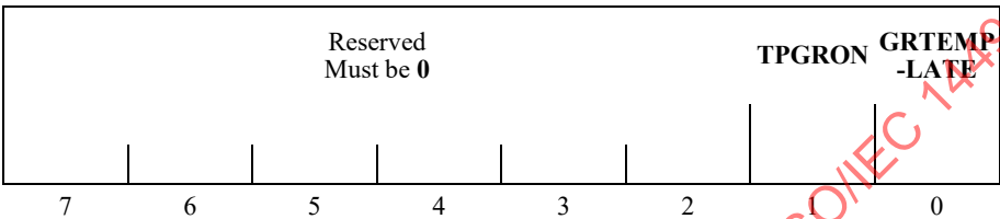
Figure 53 – Generic refinement region segment flags field structure
