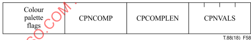
Figure 58 – Colour palette segment data header structure
