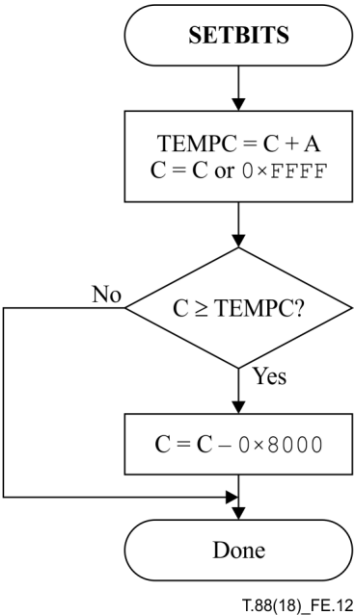
Figure E.12 – Setting the final bits in the C register
