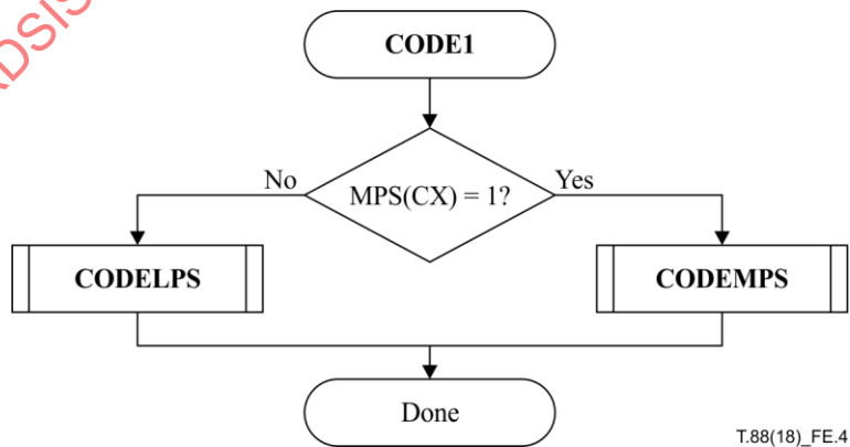
Figure E.4 – CODE1 procedure
