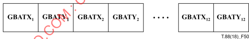
Figure 50 – Generic region AT flags field structure when GBTEMPLATE is 0 and EXTTEMPLATE is 1
