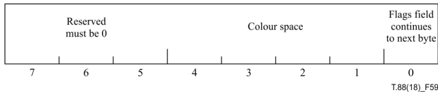
Figure 59 – Structure of the first byte of colour palette flags
