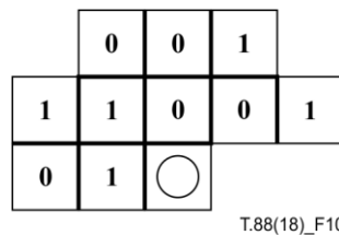
Figure 10 – Reused context for coding the SLTP value when GBTEMPLATE is 2
