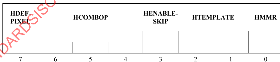
Figure 44 – Halftone region segment flags field structure
