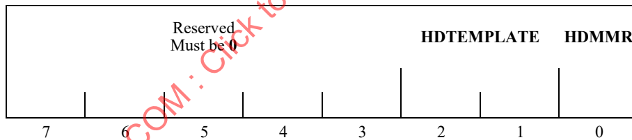
Figure 42 – Pattern dictionary flags field structure
