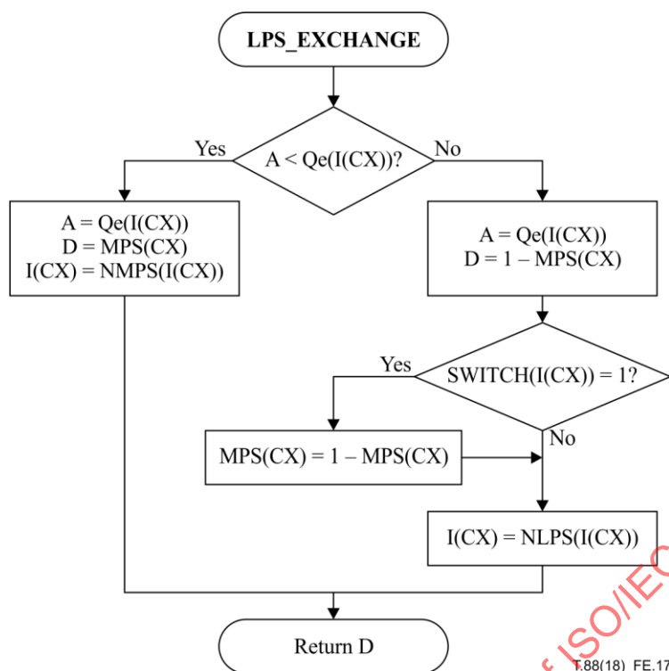
Figure E.17 – Decoder LPS path conditional exchange procedure
