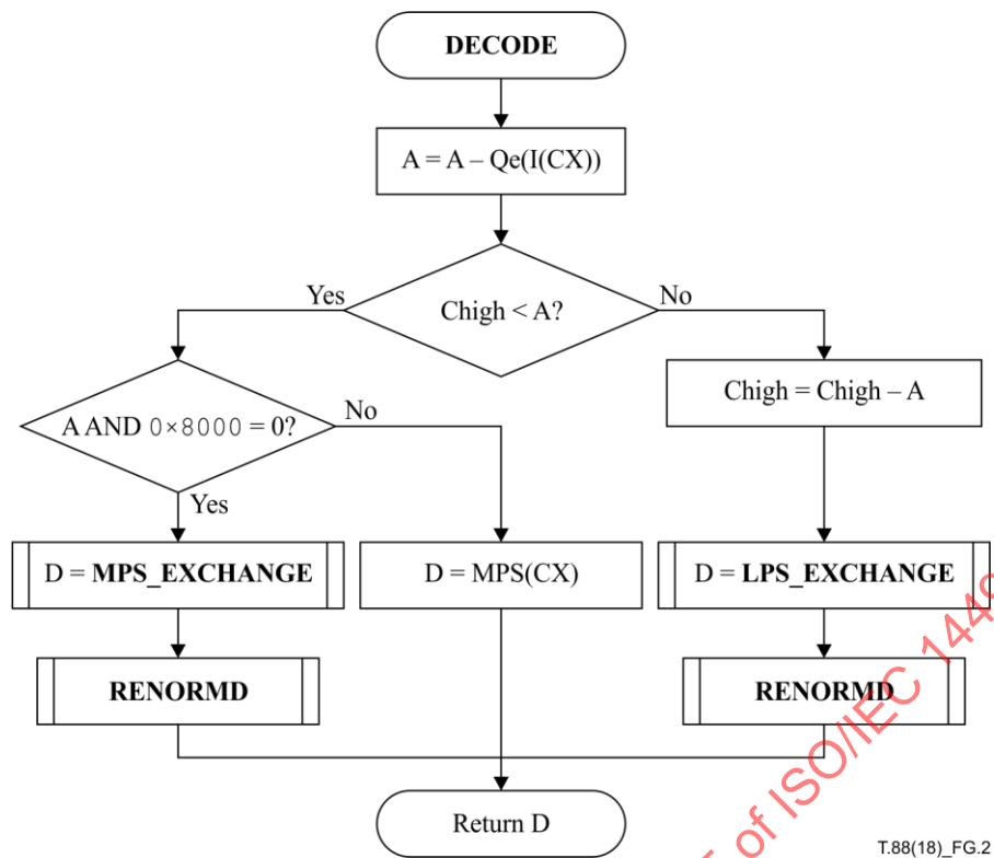
Figure G.2 – Decoding an MPS or an LPS in the software-conventions decoder
