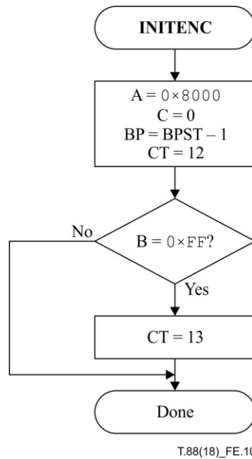
Figure E.10 – Initialization of the encoder
