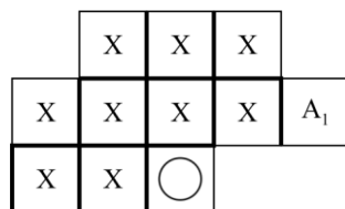
Figure 4 – Template when GBTEMPLATE = 1 showing the AT pixels at its nominal location
