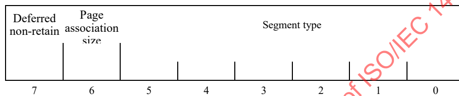
Figure 28 – Segment header flags
