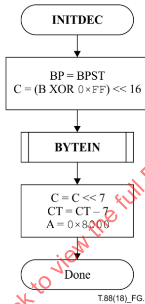
Figure G.1 – Initialization of the software conventions decoder
