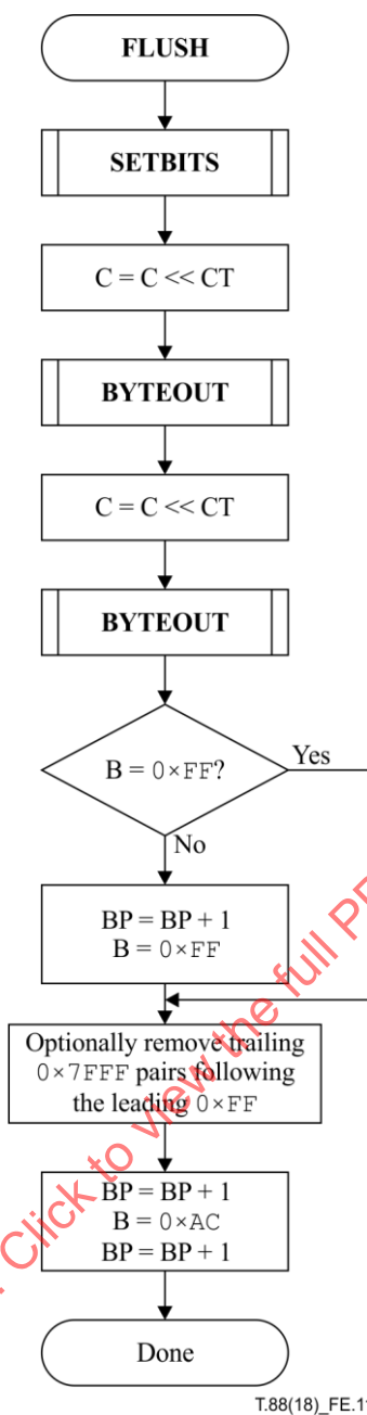
Figure E.11 – FLUSH procedure
