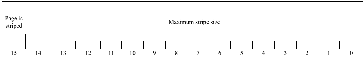
Figure 57 – Page striping information field structure
