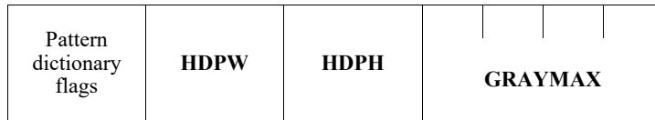
Figure 41 –Pattern dictionary header structure
