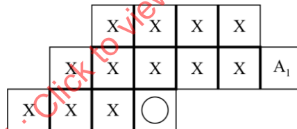
Figure 4 – Template when GBTEMPLATE = 1 showing the AT pixels at its nominal location
