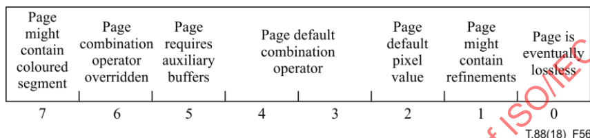
Figure 56 – Page segment flags field structure
