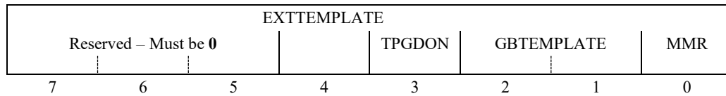
Figure 48 – Generic region segment flags field structure
