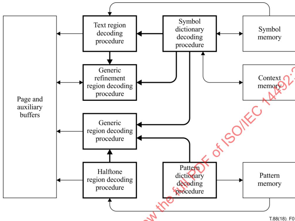
Figure 1 – Block diagram of major decoder components
