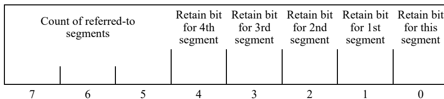
Figure 29 – Referred-to segment count and retention flags – short form
