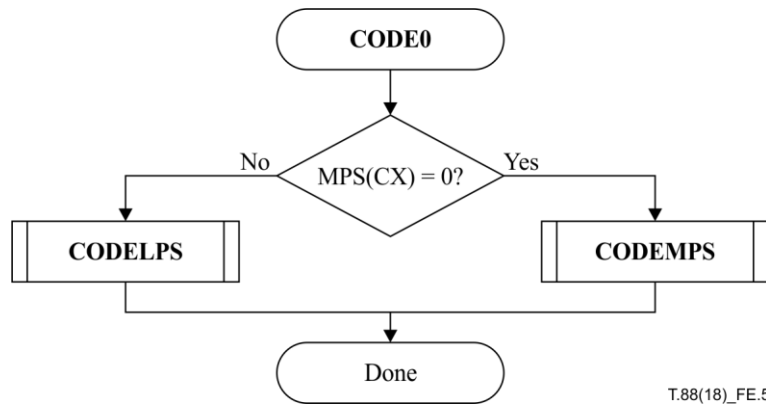
Figure E.5 – CODE0 procedure
