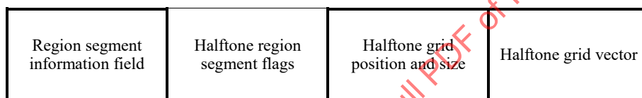
Figure 43 – Halftone region segment data header structure
