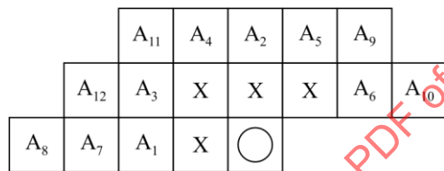
Figure 3(a) – Template when GBTEMPLATE = 0 and EXTTEMPLATE = 0, showing the AT pixels at their nominal locations
