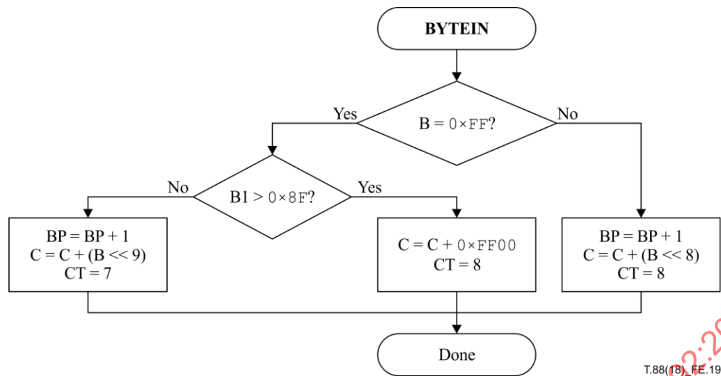
Figure E.19 – BYTEIN procedure for decoder
