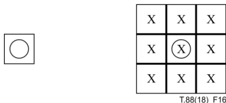
Figure 16 – TPGR template
