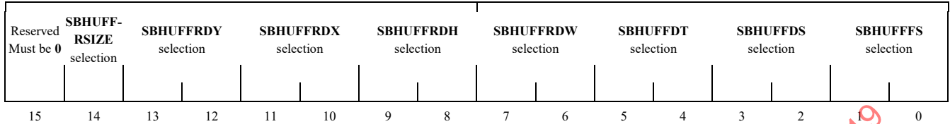
Figure 39 – Text region Huffman flags field structure
