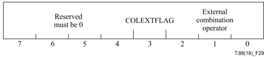
Figure 31 – Region segment flags field structure
