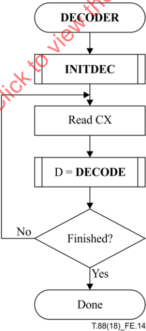
Figure E.14 – Decoder for the MQ-coder
