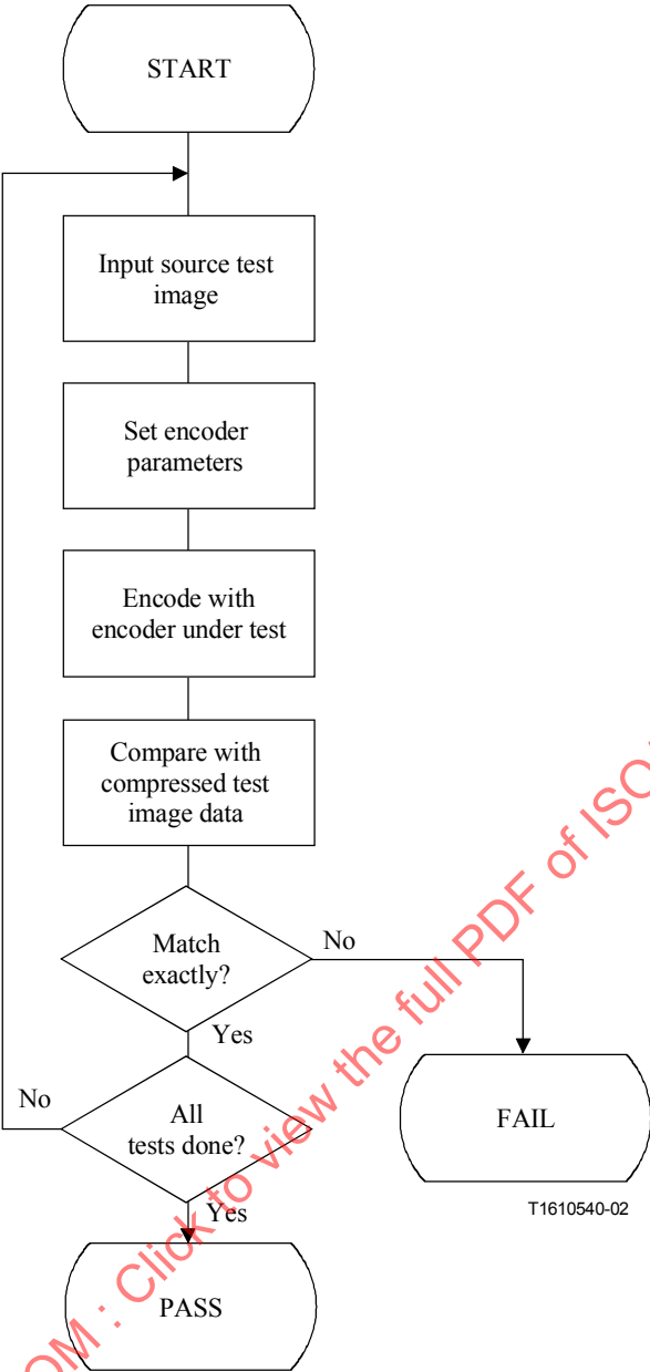
Figure 1 – Encoder testing procedure
