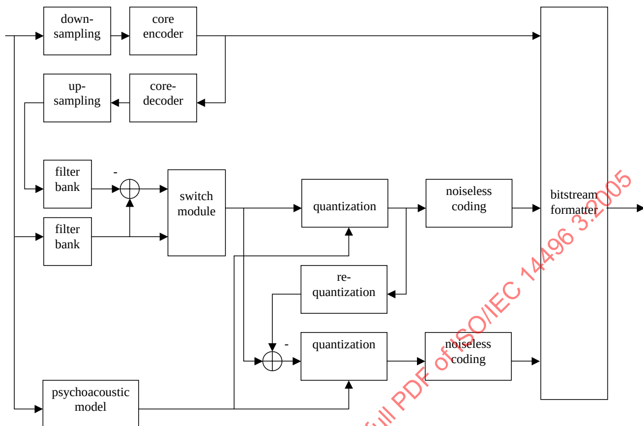
Figure 4.B.4 – Encoder process
