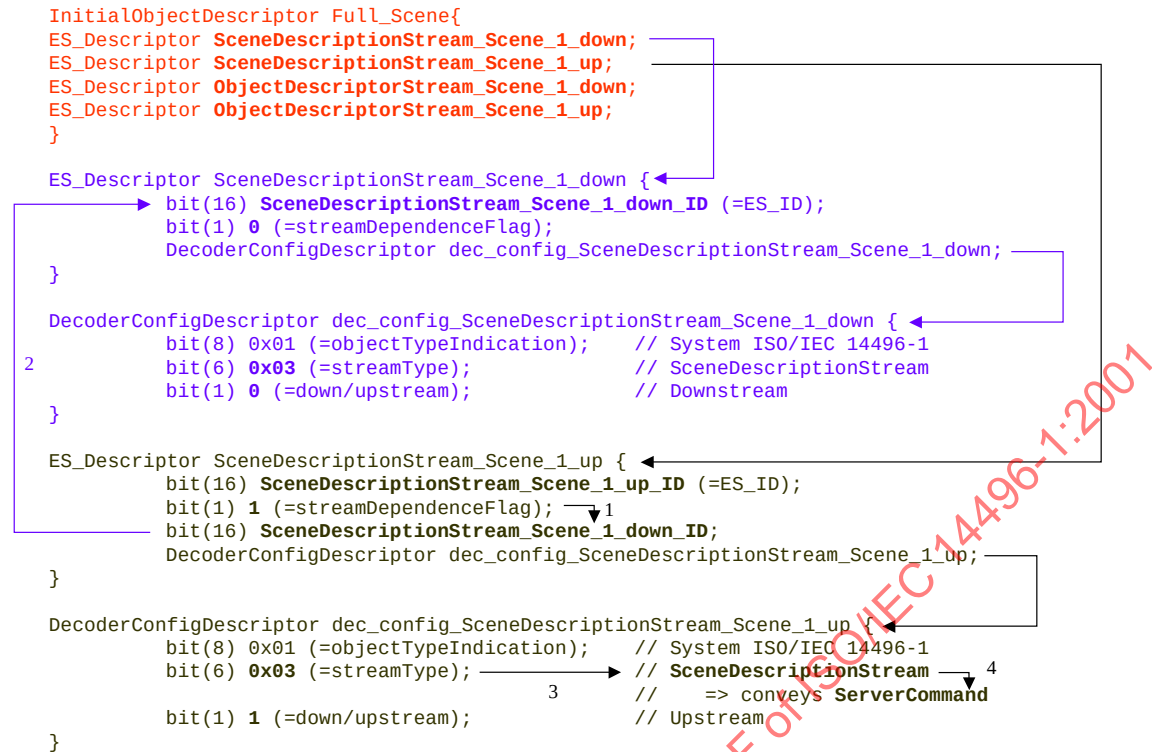
Figure 44 - Syntax for SceneDescription streams
