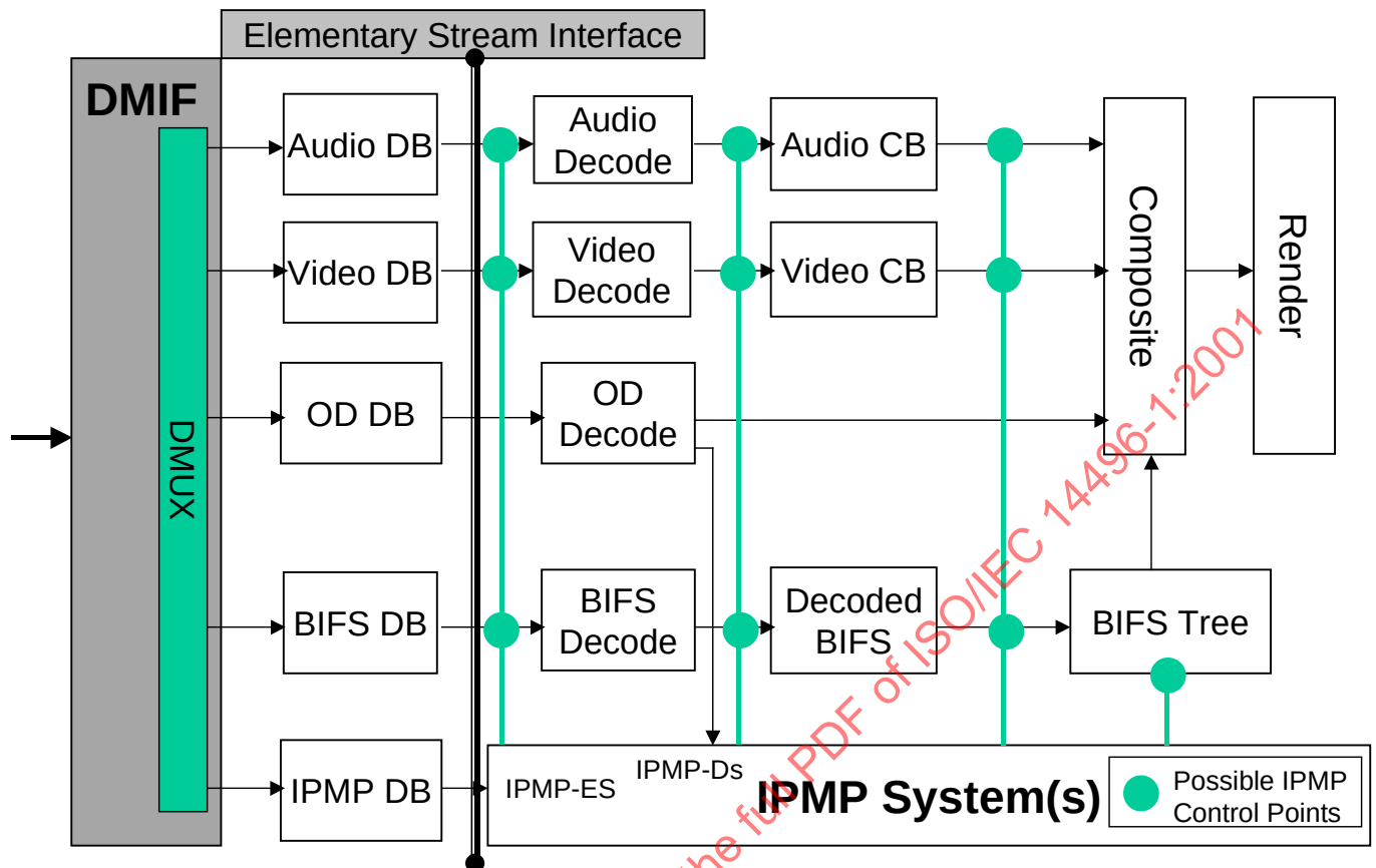
Figure 9 - IPMP system in the ISO/IEC 14496 terminal architecture
