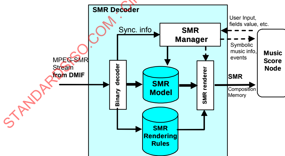
Figure 47 — SMR Decoder Block Diagram
