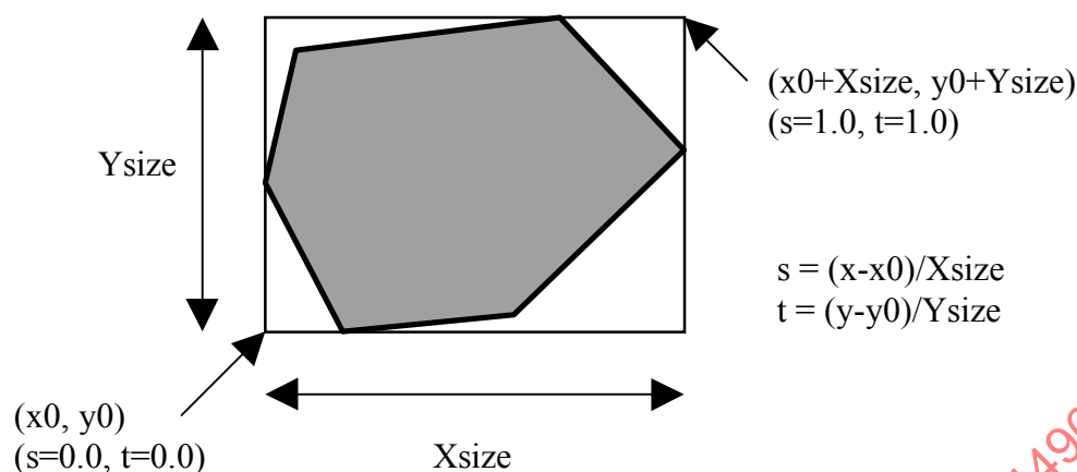
Figure 21 — IndexedFaceSet2D default texture mapping coordinates for a simple shape
