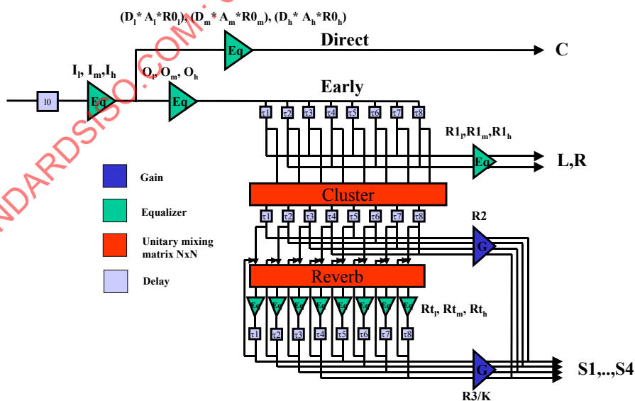
Figure 44 — Block diagram of the Room module
