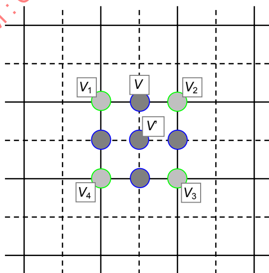
Figure COR1.2 — Computation of the offsets for the type2 quadrilateral MeshGrid.
