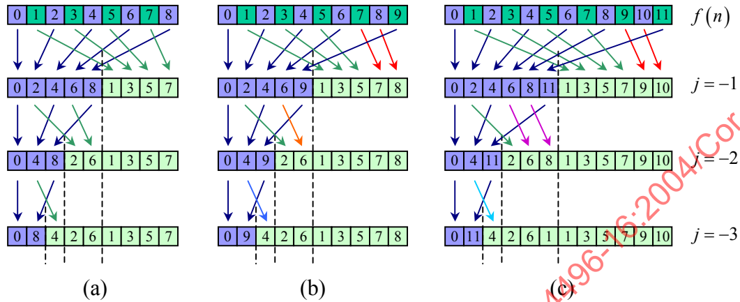
Figure 38 — Graphical illustration of the wavelet decomposition for odd and even-length signals.
