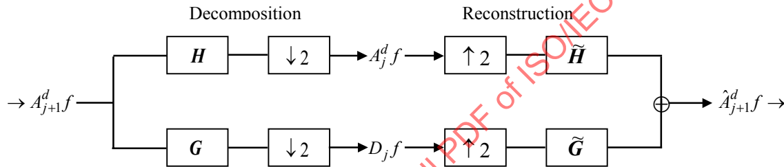
Figure 37 — Wavelet decomposition and reconstruction of a 1D signal.
