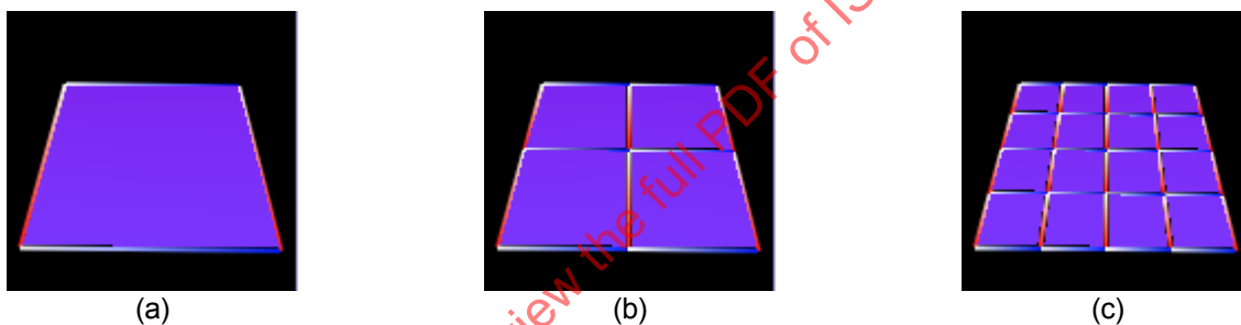
Figure COR1.1 — Example of a multi-resolution mesh with the connectivity-wireframe obtained by uniformly splitting each quad recursively into four sub-quads.
