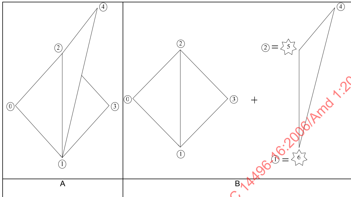
Figure AMD1-11 — A non-manifold 3D mesh (A) and converted manifold meshes (B)
