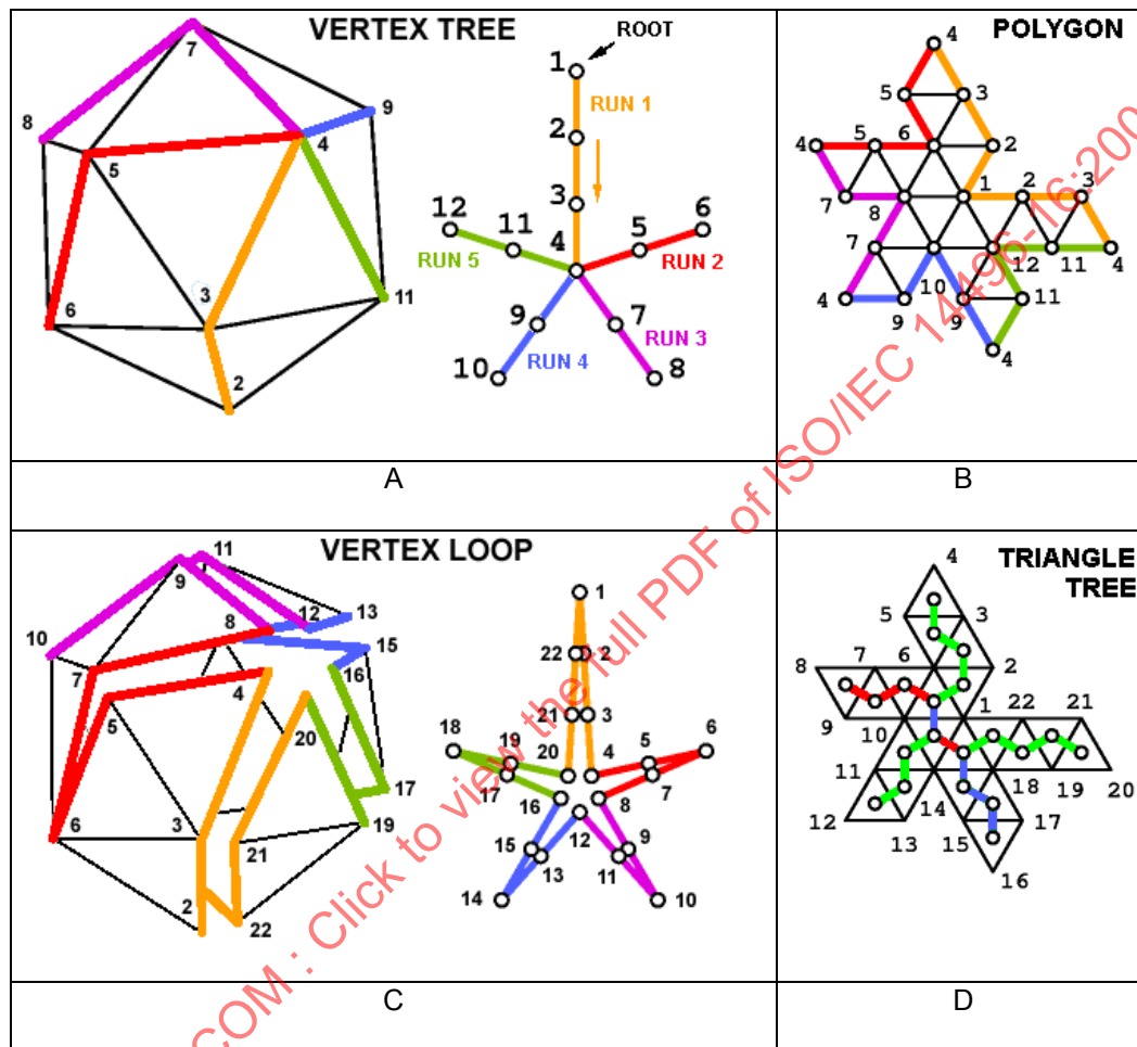
Figure AMD1-7 — Topological Surgery representation of a simple mesh.
