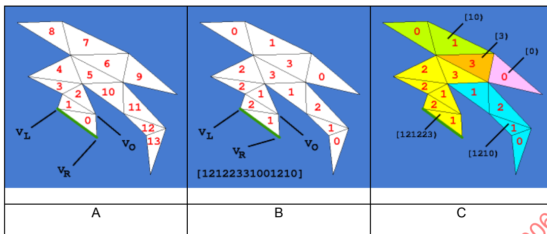
Figure AMD1-10 — Representing a simple polygon as a table of triangle runs.
