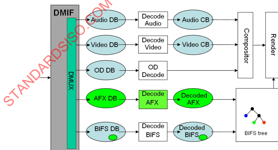
Figure 1 — Animation Framework eXtension (in green) and MPEG-4 Systems.
