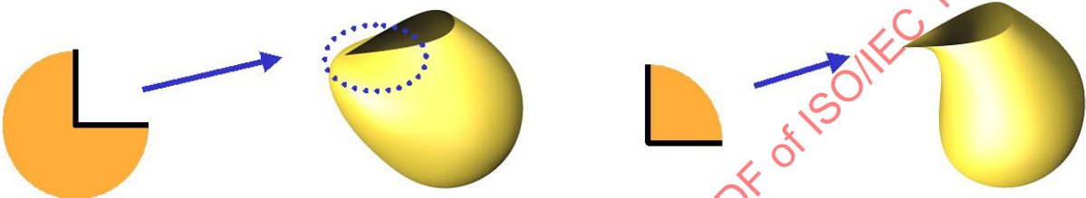
Figure 16 — Concave corners (left) and convex corners (right).
