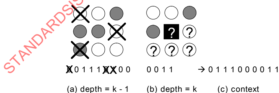
Figure 70 — Example of context: a voxel represented by a question marked black square in (b) is the voxel to be decoded and voxels represented by white circles and gray circles in (a) and (b) are used to make a context excluding three voxels which are marked with 'X'.
