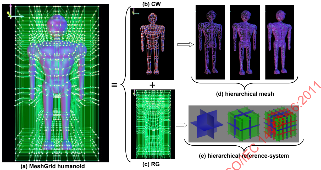
Figure 20 — A MeshGrid humanoid model designed by means of implicit surfaces.
