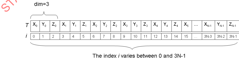
Figure 65 — Example of a flat representation of an array of quantized position coordinates.
