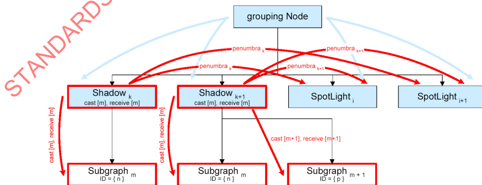
Figure 31 — Transmission of shadow properties to multiple 3D-surfaces and light sources
