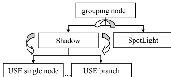
Figure 29 — Semantical representation
