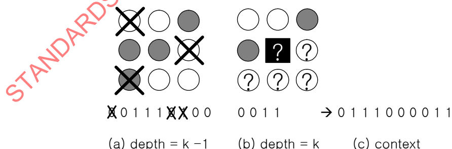
Figure 74 — Example of context: a voxel represented by a question marked black square in (b) is the voxel to be decoded and voxels represented by white circles and gray circles in (a) and (b) are used to make a context excluding three voxels which are marked with 'X'.
