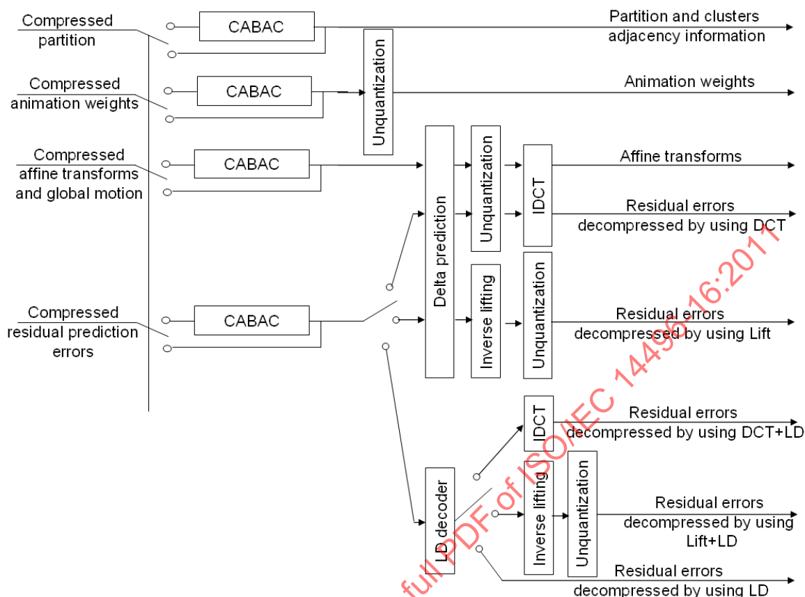
Figure 80 — FAMC decoding process.
