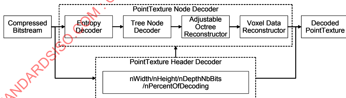
Figure 67 — Block diagram of decoder for PointTexture compression.
