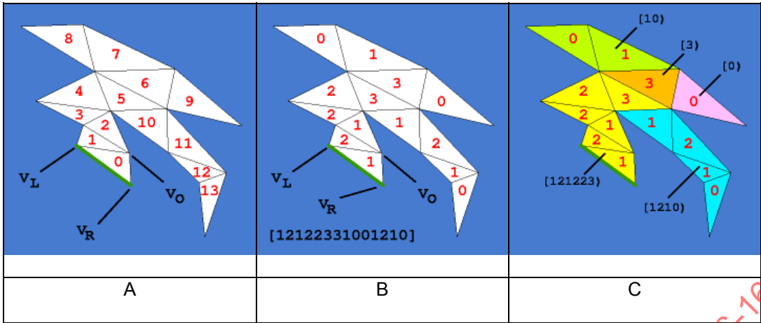
Figure 38 — Representing a simple polygon as a table of triangle runs. A: depth-first order of traversal of the triangle tree starting from the root edge (green). B: each triangle is classified by a 2-bit code as leaf (0), advance-right (1), advance-left (2), or branching (3). C: The sequence of 2-bit codes is partitioned into runs ending in branching or leaf triangles. Each run is encoded as a (tt_run_length,tt_leaf) pair, plus a sequence of marching_edge bits. Optionally, in the case of 3D meshes with polygonal faces, an additional sequence of polygon_edge bits is used to indicate which internal edges of the simple polygon correspond to original internal edges of the mesh, and which ones to virtual internal edges.
