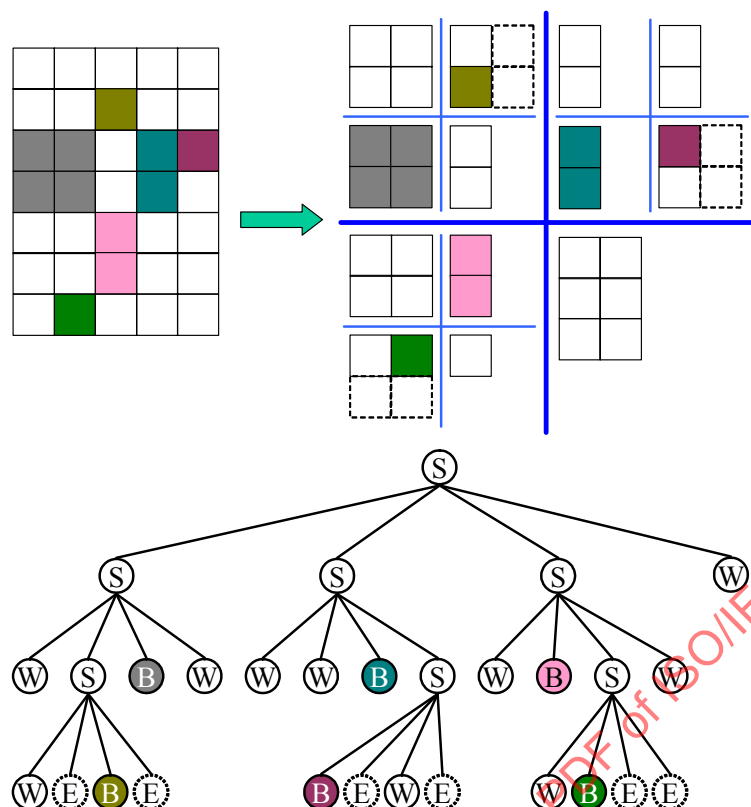
Figure 69 — Example of adjustable octree in the resolution of 5×7.
