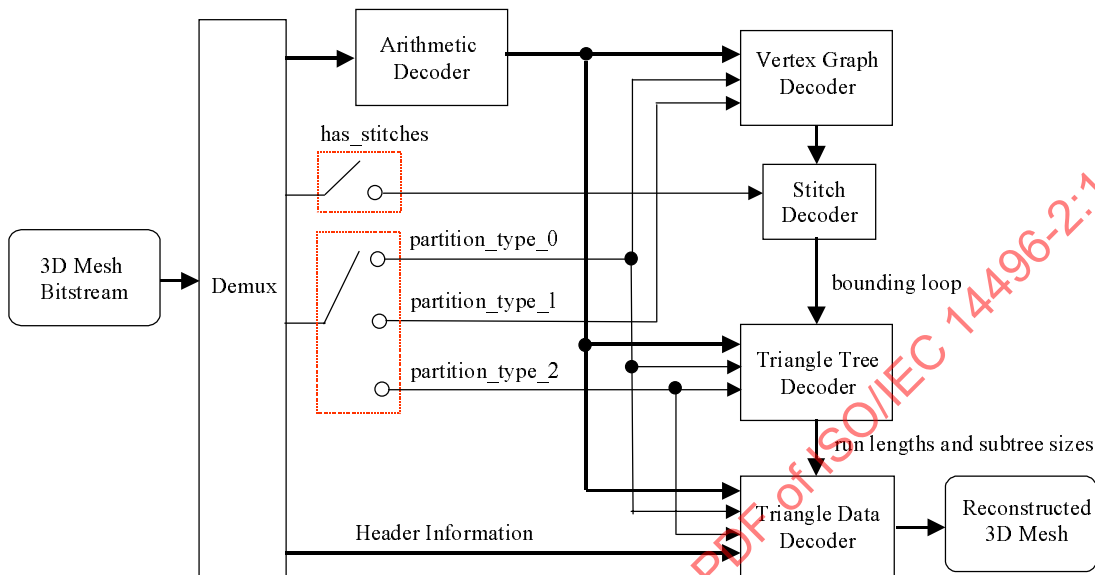
Figure V2 - 40 -- Block diagram of the Topological Surgery decoder
