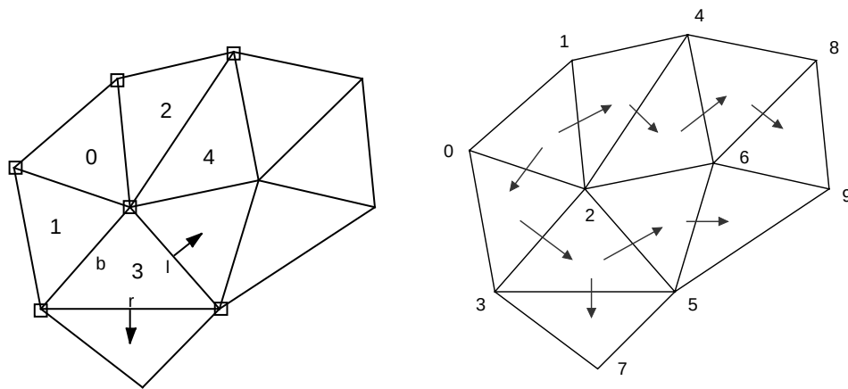
Figure 7-46 -- Breadth-first traversal of a 2D triangular example mesh
