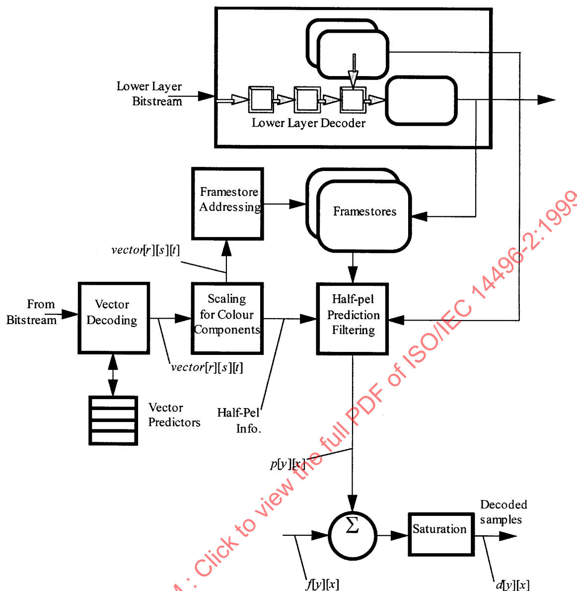
Figure 7-33 -- Simplified motion compensation process for temporal scalability
