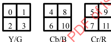
Figure AMD1-5 — 4:4:4 Macroblock structure
