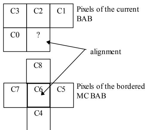
Figure V2 - 16 -- The templates of Inter-mode CAE for enhancement layer. C6 is aligned with the pixel to be decoded. The pixel to be decoded is marked with '?'. STANDARDISO.COM : Click to view the full PDF of ISO/IEC 14496-2:2001
