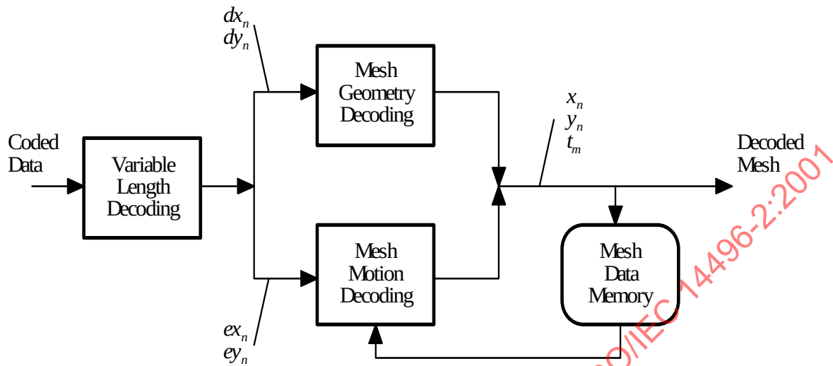
Figure 7-41 -- Simplified 2D Mesh Object Decoding Process
