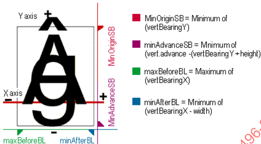
Figure 2 – Vertical text
