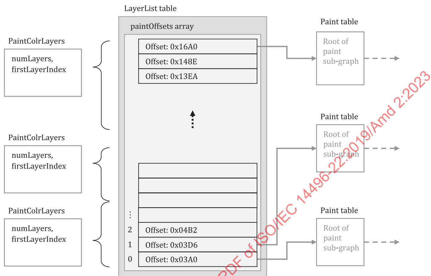
Figure 5.37 — Version 1: PaintColrLayers tables specify slices within the LayerList, providing a layering of content defined in sub-graphs.
