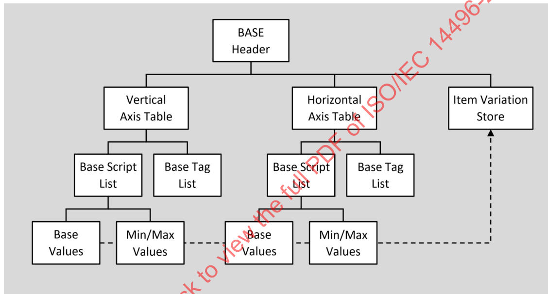
Figure 6.17 – High-level organization of BASE table
