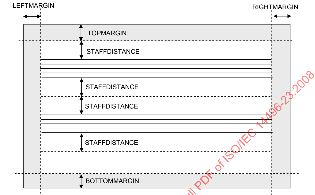
Figure 3 — FORMATPAGECOMPUTERVIEW parameters
