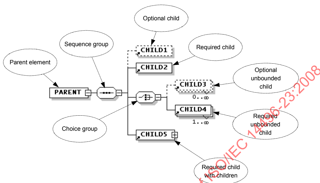
Figure 1 — Example element syntax diagram
