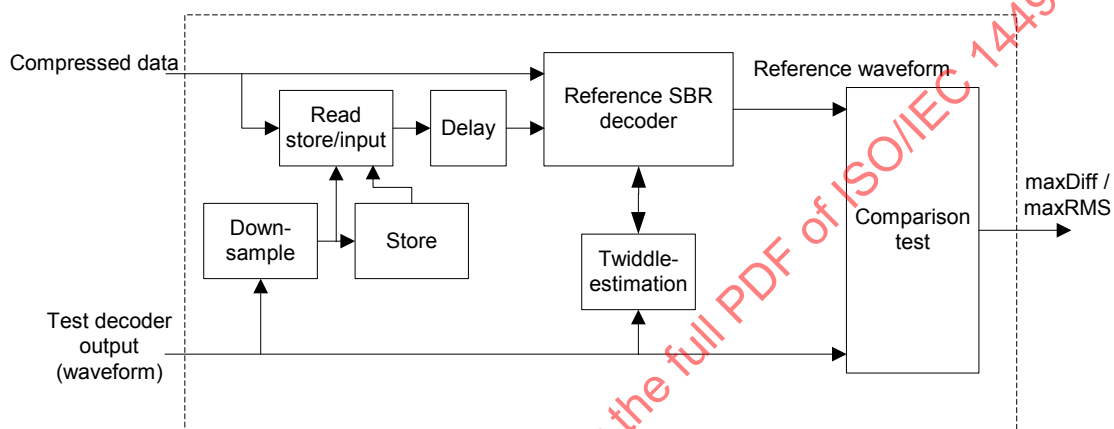
Figure 11 — Block diagram of the SBR conformance test procedure
