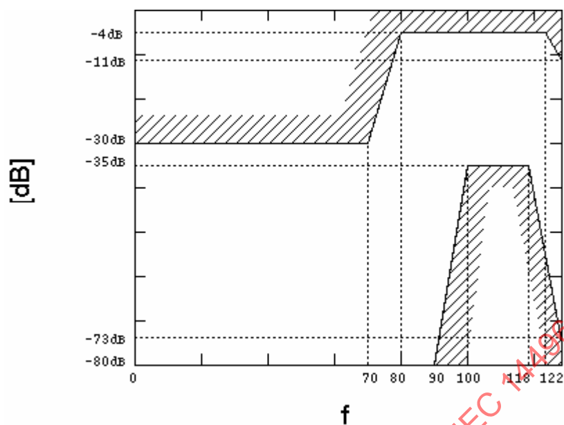
Figure 5 — Acceptable range of differential spectrum (for bitstream HV01)
