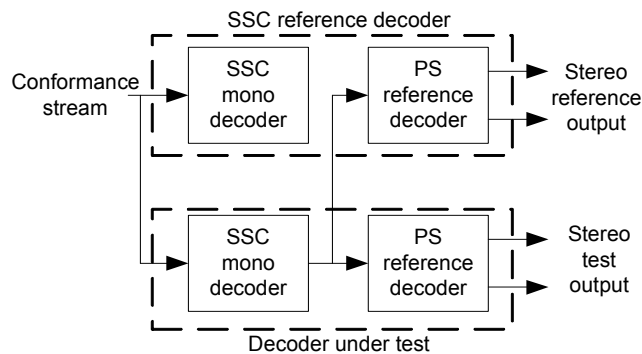
Figure 12 — Parametric stereo conformance setup.
