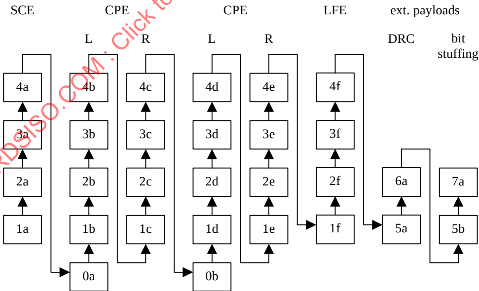
Figure 31: Dependency structure in case of error resilient multichannel AAC syntax (channelConfiguration == 6)
