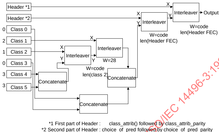
Figure 29: Interleave process with class-wise control of interleaving
