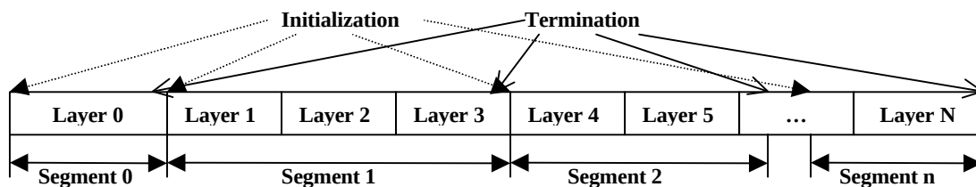
Figure 11: The structure of SBA coded bitstream
