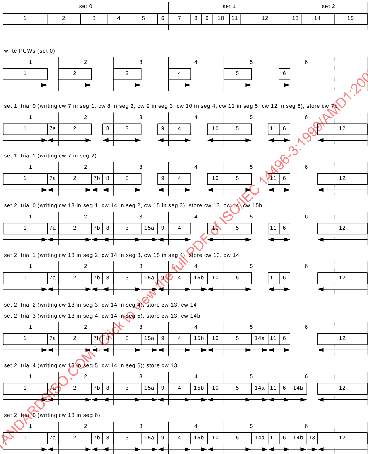
Figure 16: Example for HCR encoding algorithm (only one segment width, pre-sorting has been done before)
