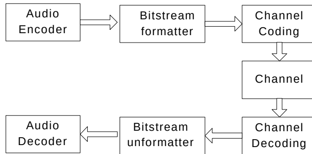
Figure 30: Basic principle of error resilient bitstream reordering
