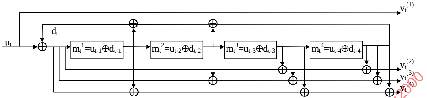
Figure 20: Shift register realization for systematic recursive convolutional encoder
