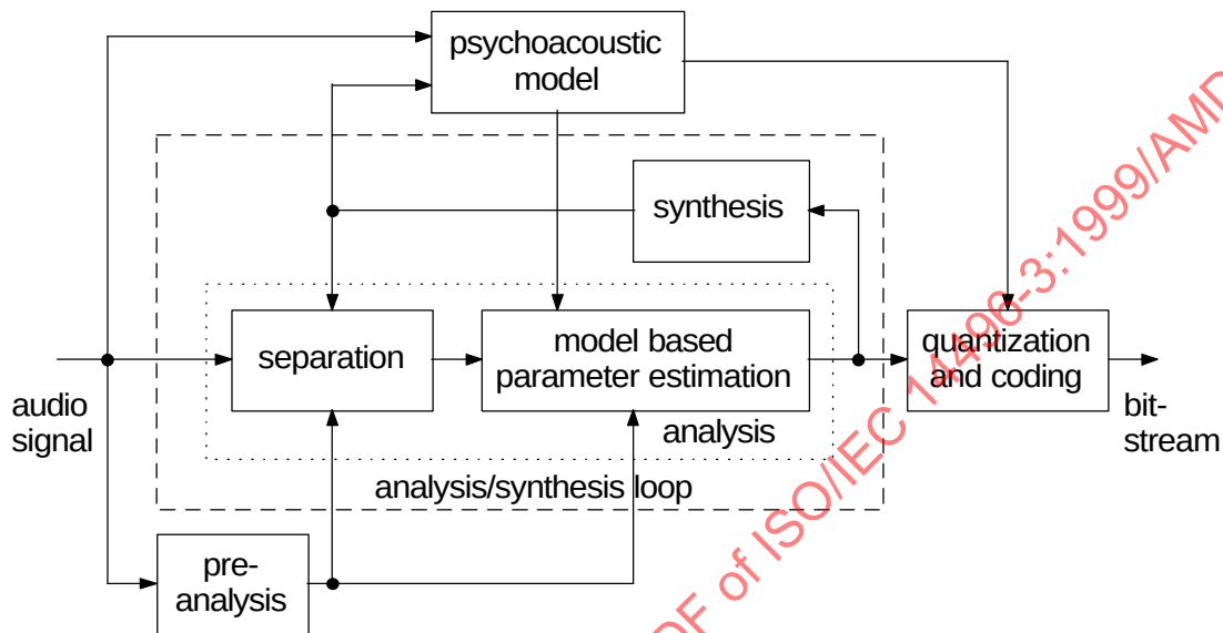
Figure A.2: Block diagram of the HILN encoder
