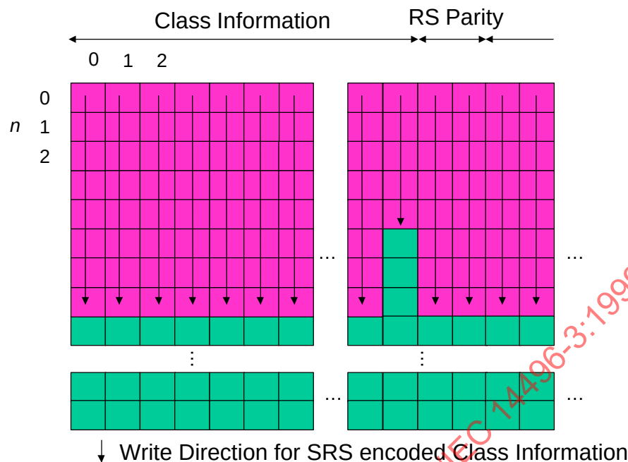
Figure 28: Interleaving matrix in RS encoded class case
