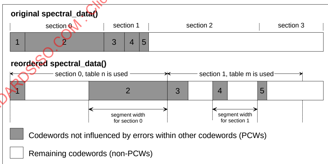
Figure 15: General scheme of segmentation and arrangement of PCWs
