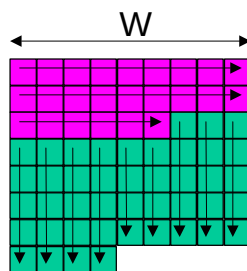
Figure 24: Interleave matrix in non-rectangular case
