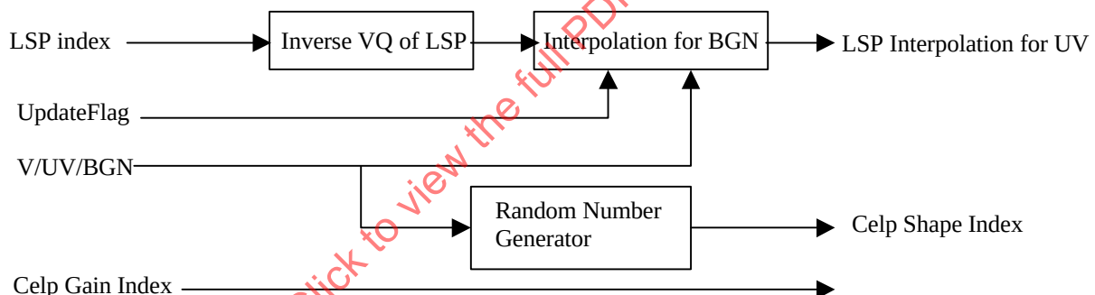
Figure 34: Additional diagram for variable rate decoder
