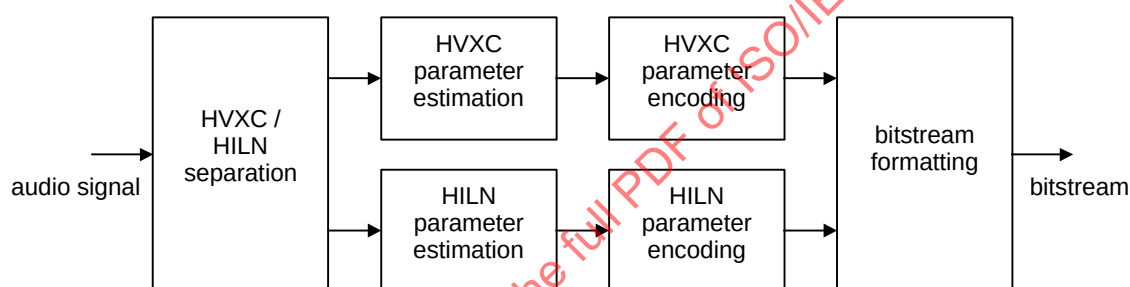
Figure A.1: General block diagram of the integrated parametric encoder
