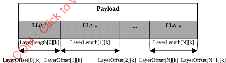
Figure 8: Structure of the payload
