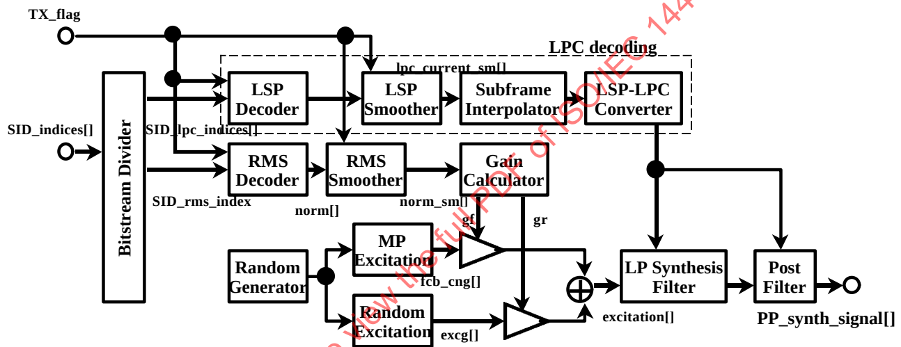
Figure 33: CNG module
