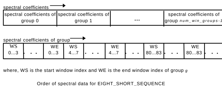
Figure 10: Order of spectral data for EIGHT_SHORT_SEQUENCE
