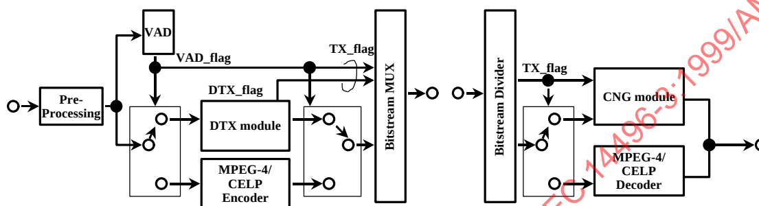
Figure 32: Block diagram of the codec system with the silence compression tool
