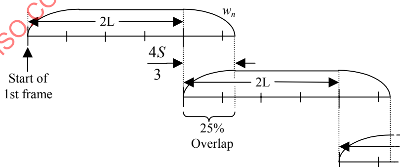
Figure 8.14 - Overlap and add. In the overlap a half Hanning window h is used. In the intermediate part the window is set to 1. The first 4 sub-frames are starting with a fade-in realised by the Hanning window
