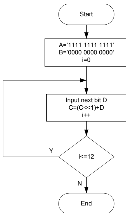
Figure 10.9 — Initialization
