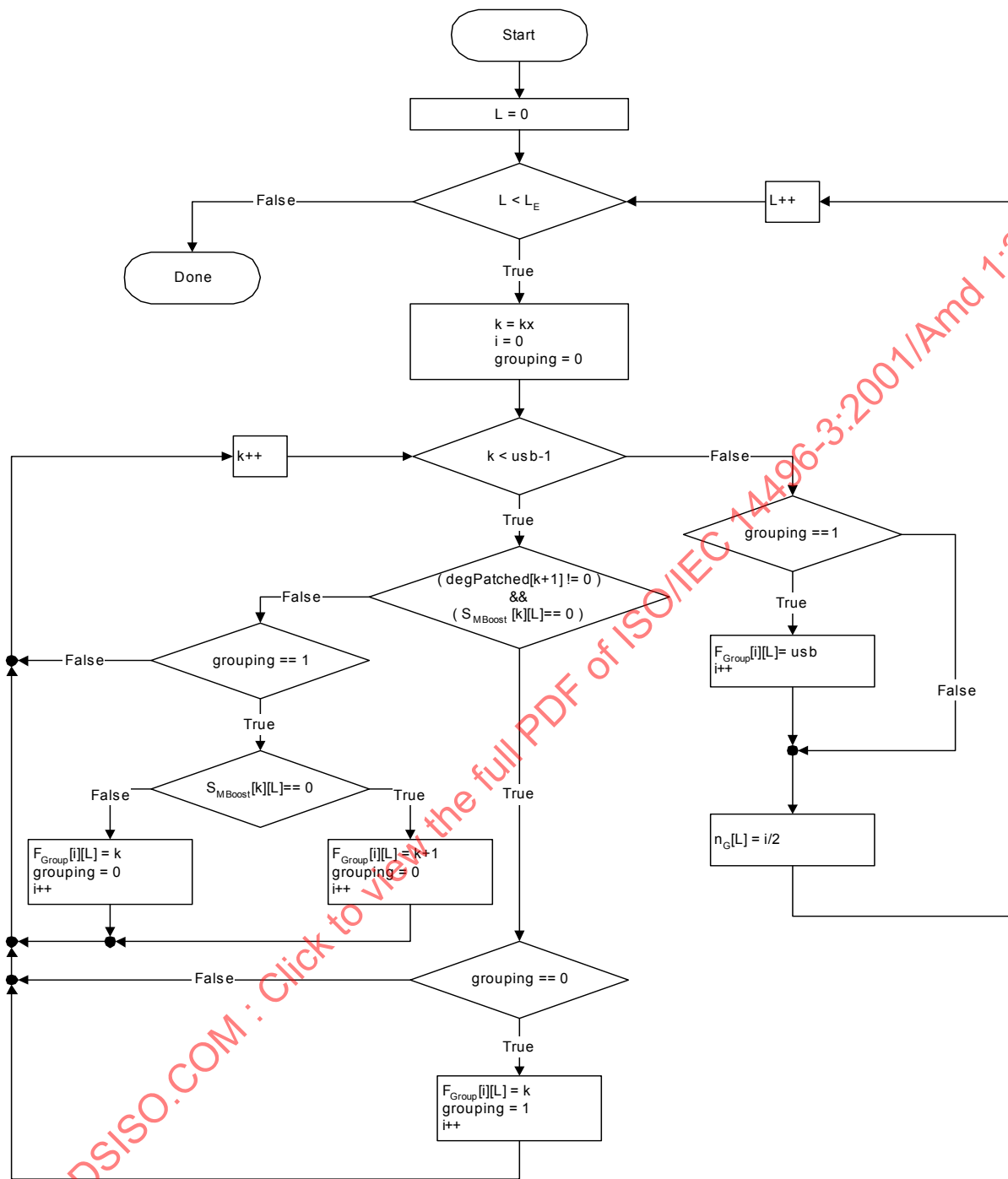
Figure 4.52 – Flowchart of the calculation of the gain groups
