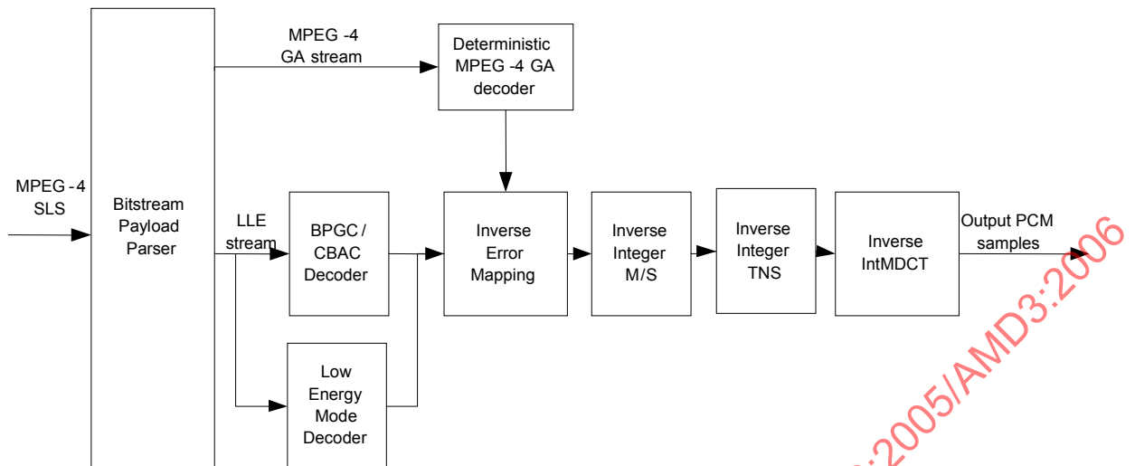
Figure 12.1 – SLS decoder block diagram
