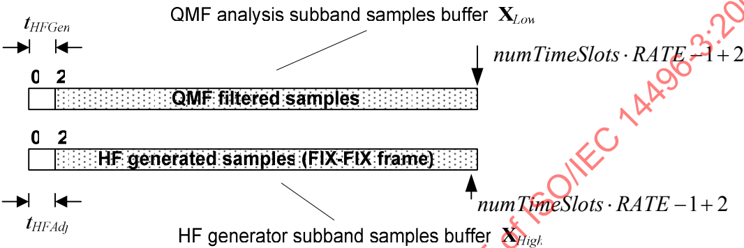
Figure AMD9.2 — Synchronization for low delay SBR
