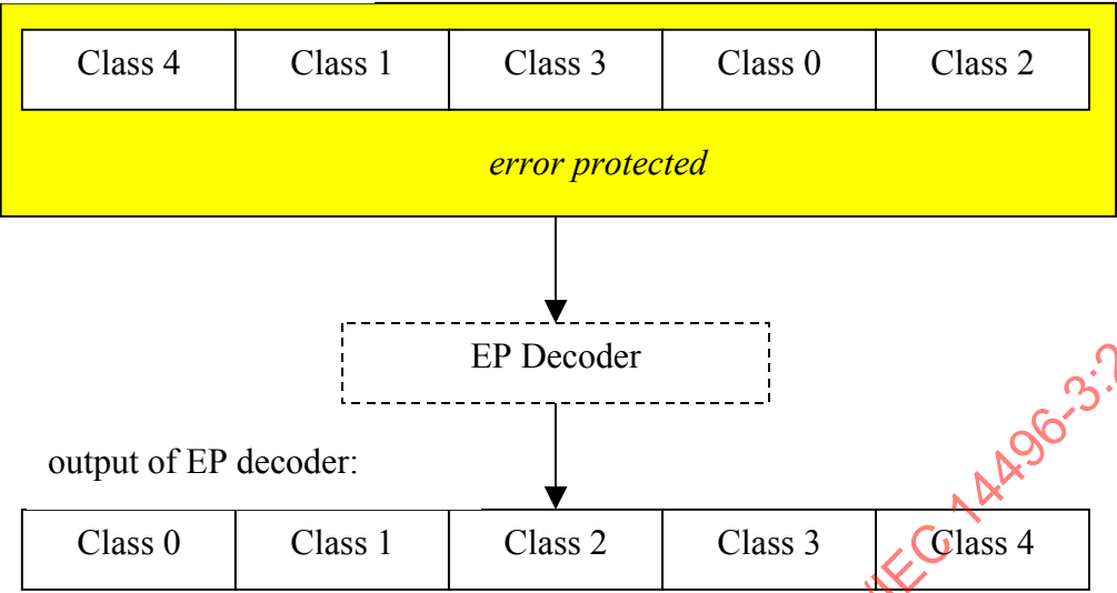
Figure 1.20 – Example for class reordered output with class_output_order 4, 1, 3, 0, 2
