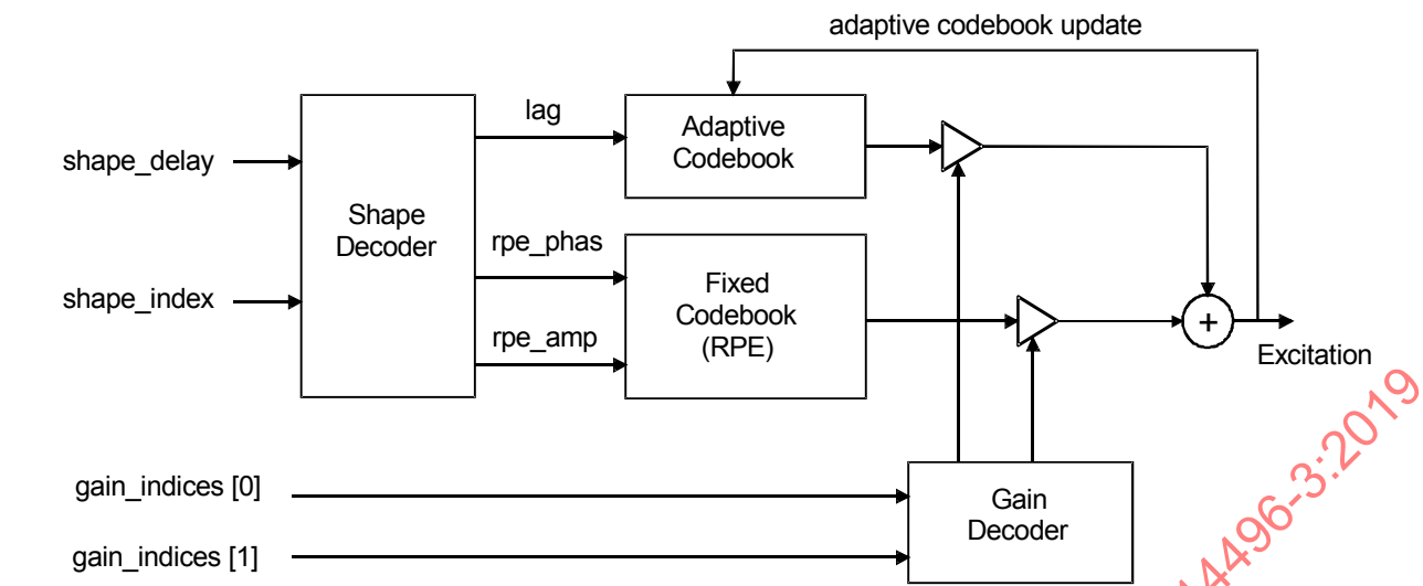
Figure 3.6 — Regular pulse excitation generator
