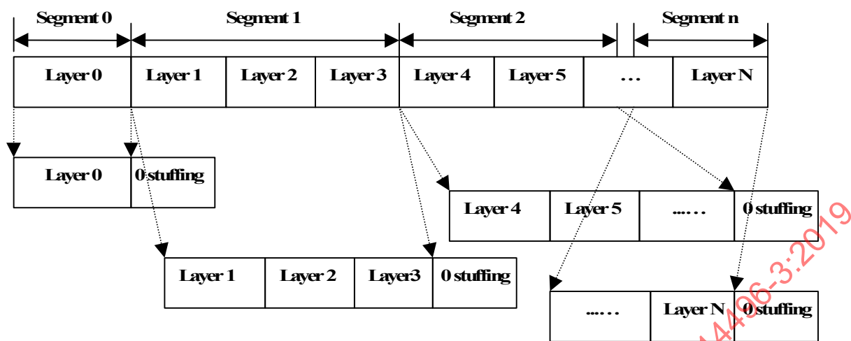
Figure 4.28 – Decoding of SBA bitstream payload
