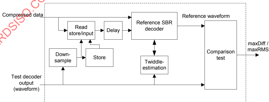
Figure AMD8-2 — Block diagram of the SBR conformance test procedure
