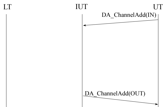
Figure 21 — Channel Add for Local Storage
