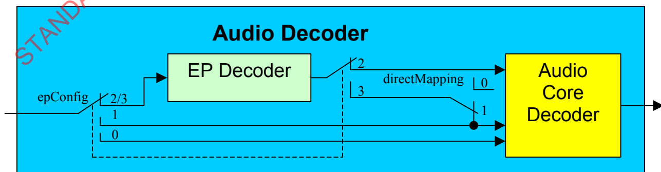
Figure 5 – Audio decoder structure
