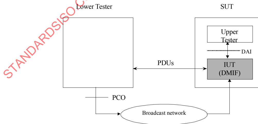
Figure 23 — The test method for the DAI test environment for a broadcast scenario
