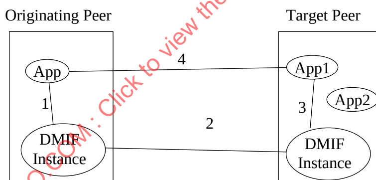
Figure 4 — DMIF computational model
