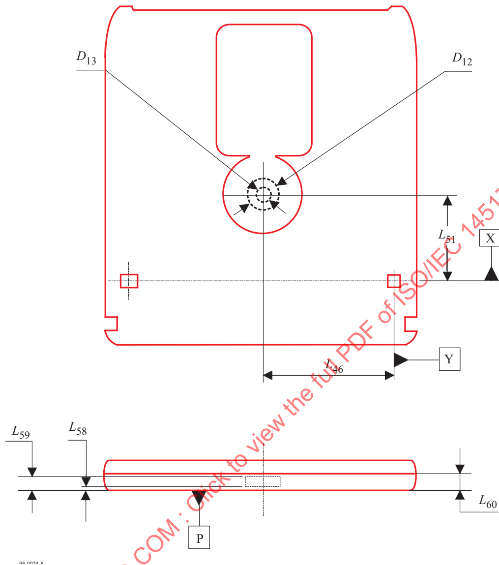
Figure 13 - Capture cylinder
