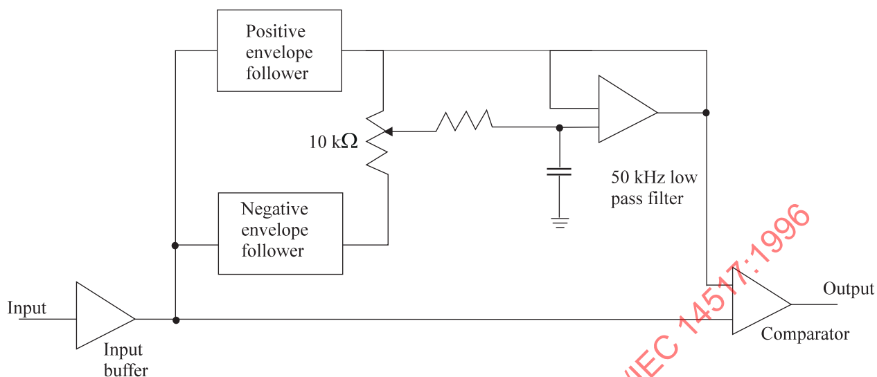
Figure H.1a - Tracking threshold block diagram
