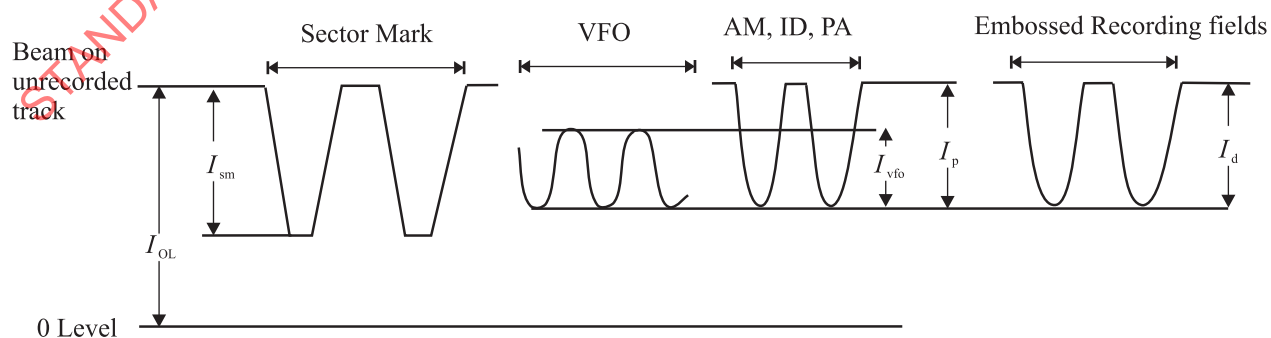
Figure 24c - Signals from Headers and embossed Recording fields in Channel 1
