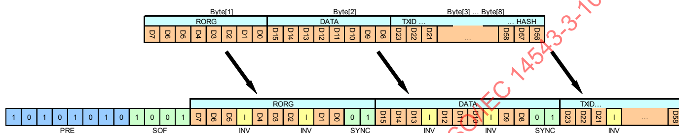
Figure 3 – Complete frame structure for the 868,3 MHz WSP protocol
