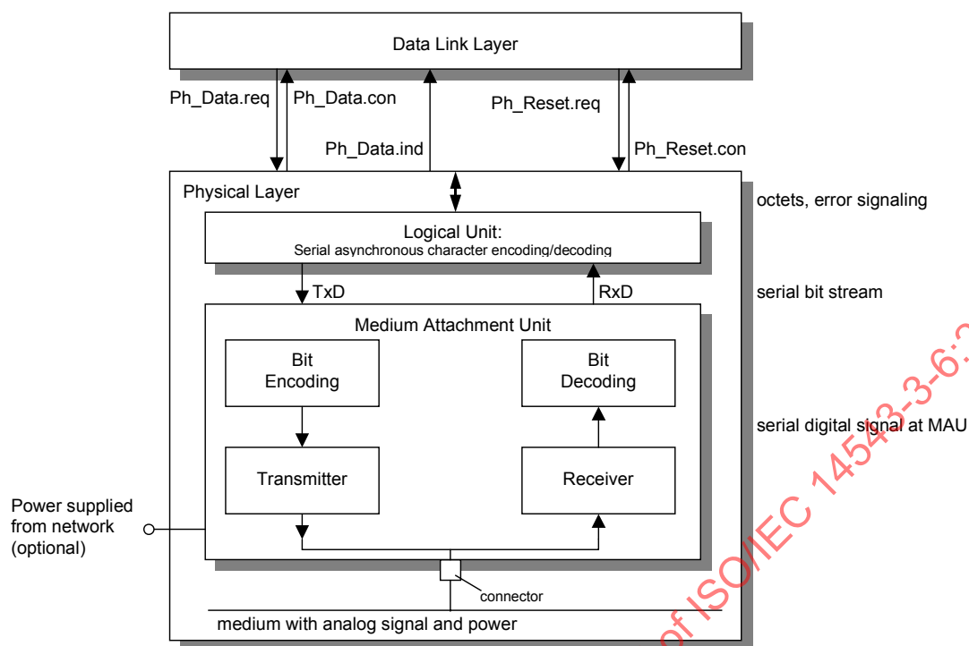
Figure 21 – Logical structure of physical layer type TP1
