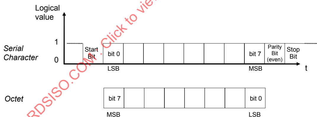
Figure 22 – Octet mapped to a serial character
