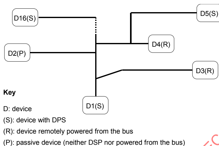
Figure 8 – TP0 Network with distributed power supply
