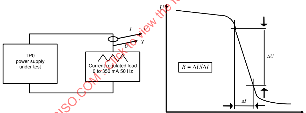
Figure 6 – Power supply dynamic internal resistor measuring test set-up
