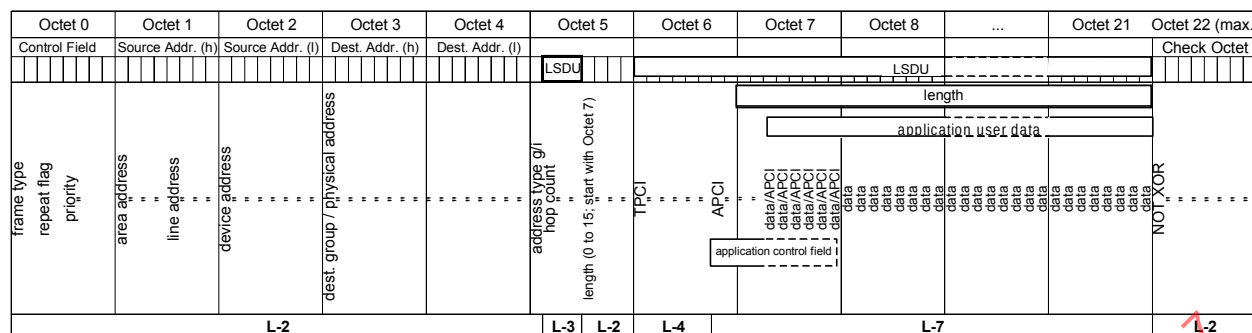
Figure 40 – Format 1s, L_Data_Standard frame format
