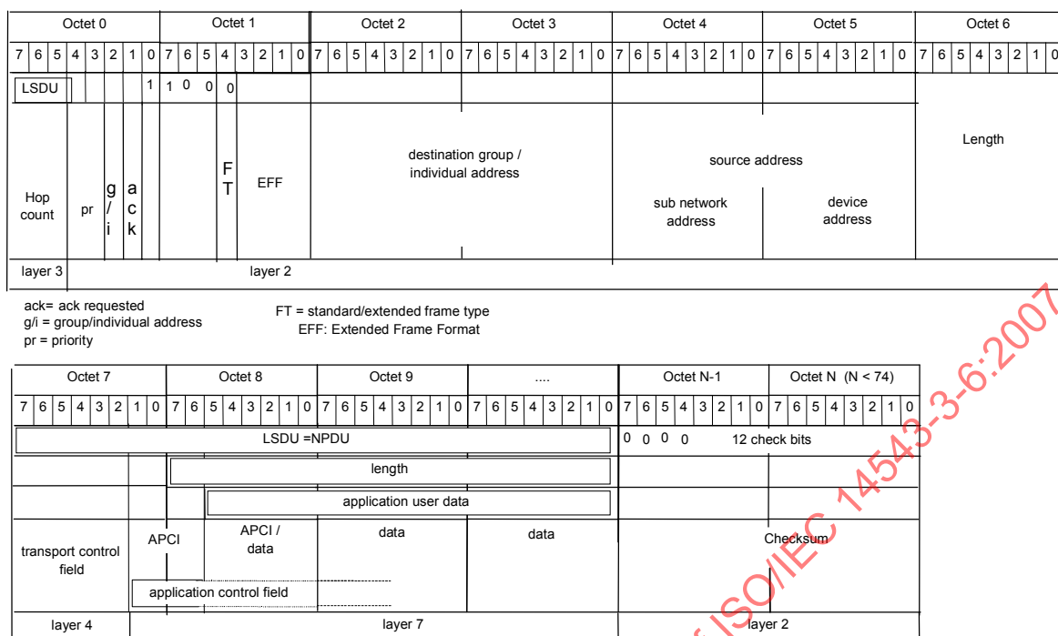
Figure 20 – Format 1e, Full L_Data_Extended request frame format
