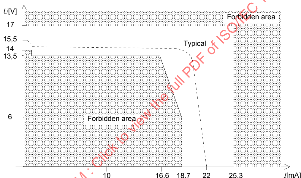
Figure 9 – Voltage/Current gauge of one node
