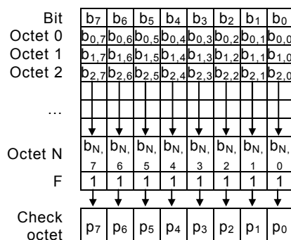
Figure 41 – Check octet
