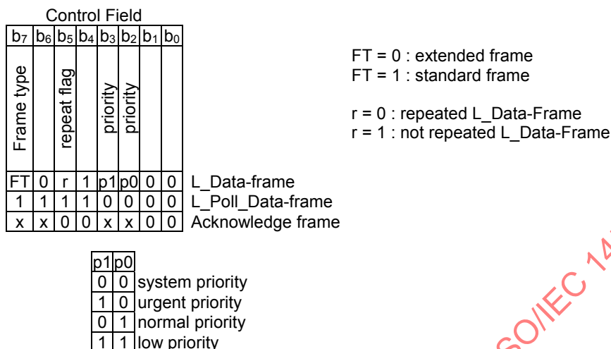
Figure 38 – Control field
