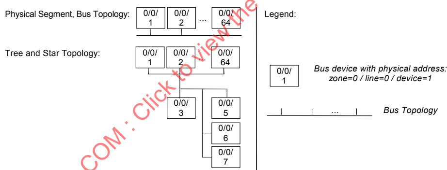
Figure 34 – Physical segments
