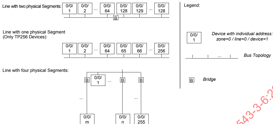
Figure 35 – Physical segments combined to a line
