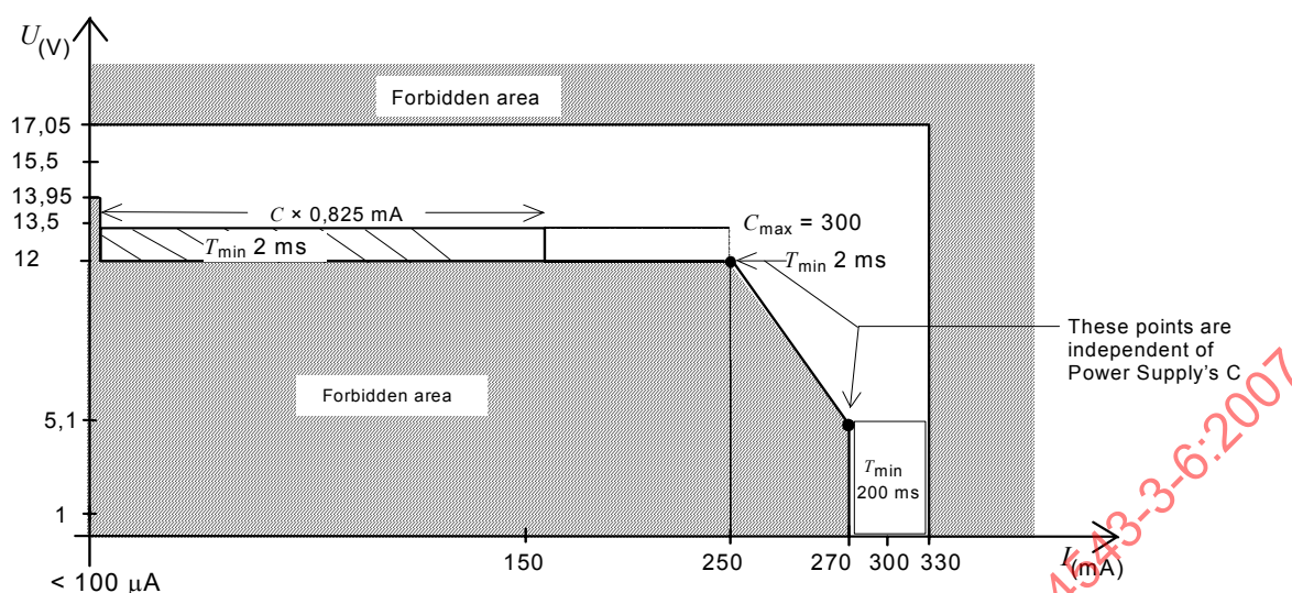
Figure 5 – TP0 power supply gauge
