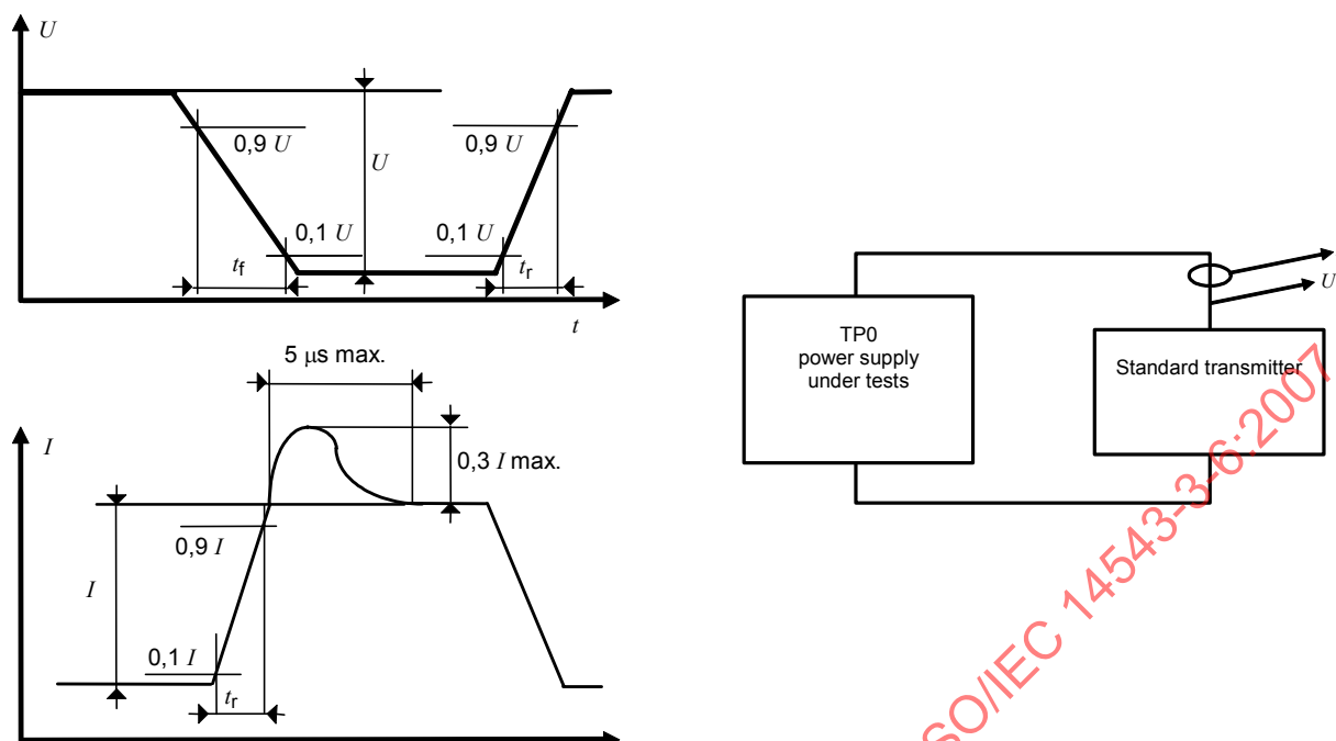
Figure 7 – Falling edge and over-current measurements
