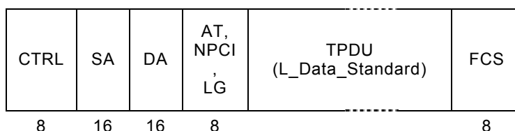
Figure 39 – Frame fields with standard fieldname abbreviations
