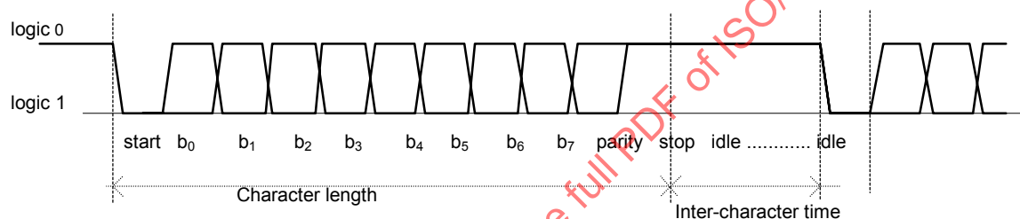
Figure 2 – Character format
