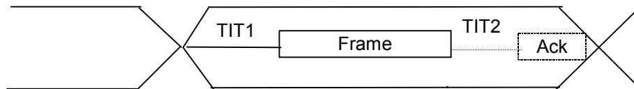
Figure 18 – Transmission definition
