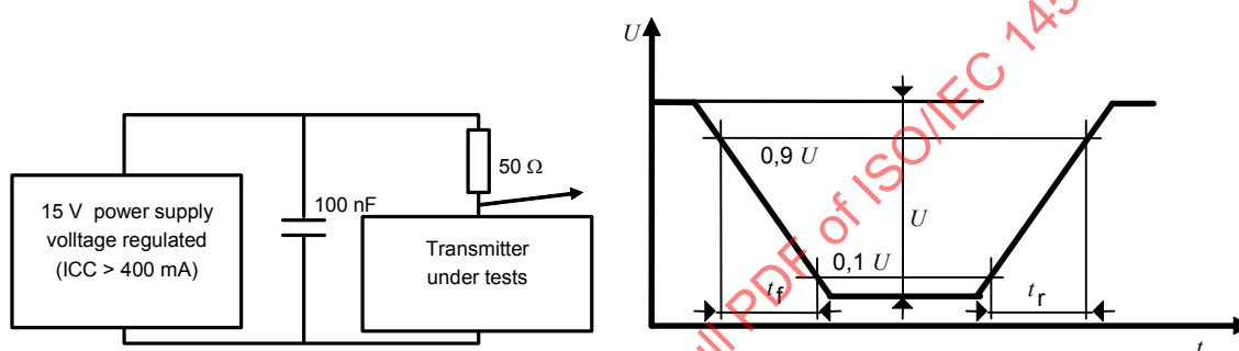
Figure 3 – Transmitter rising and falling edges
