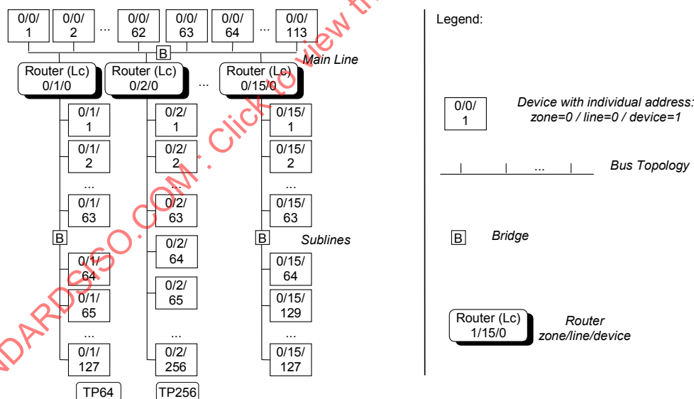
Figure 36 – Lines combined to a zone
