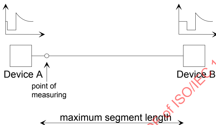
Figure 25 – Delayed logical “0”
