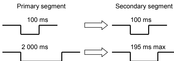
Figure 4 – Repeater maximum transition time
