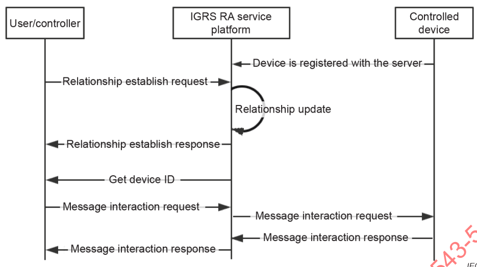
Figure 8 – Controller–IRSP–device WAN interaction process
