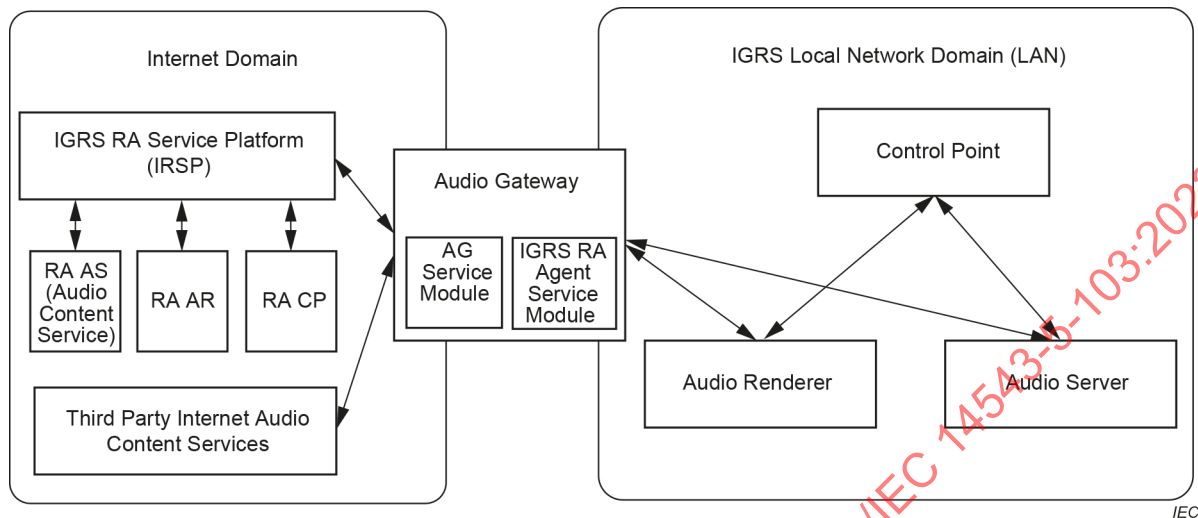
Figure 1 – RA smart audio interconnection system architecture
