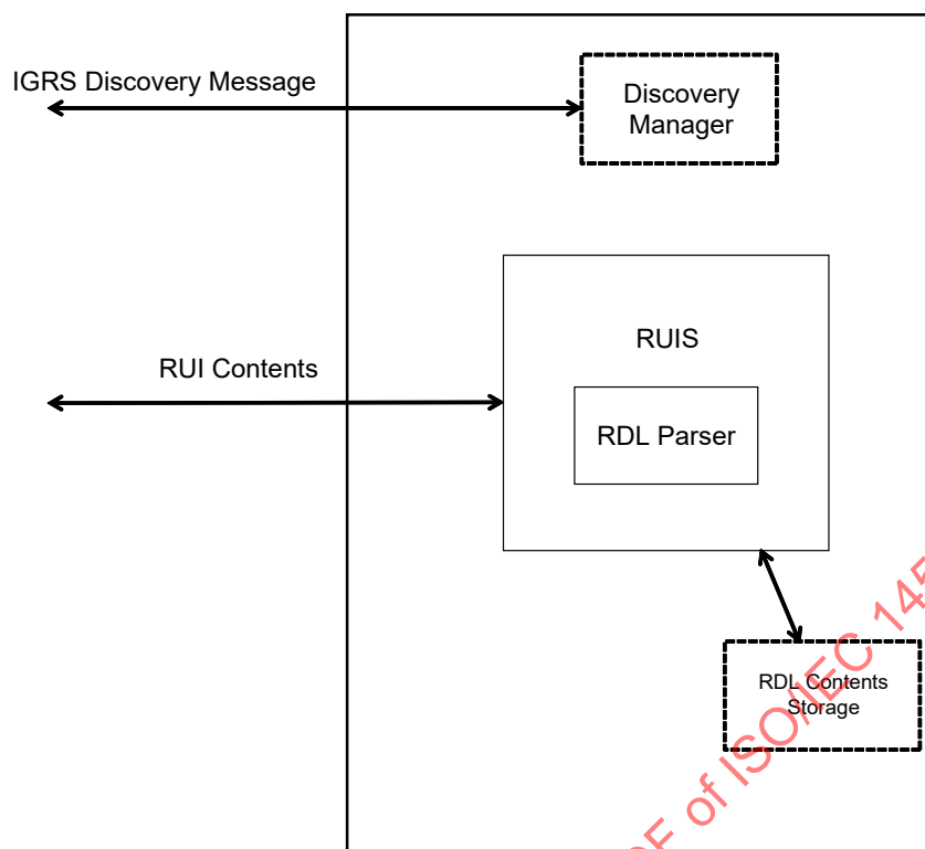
Figure 6 – RUIS architecture
