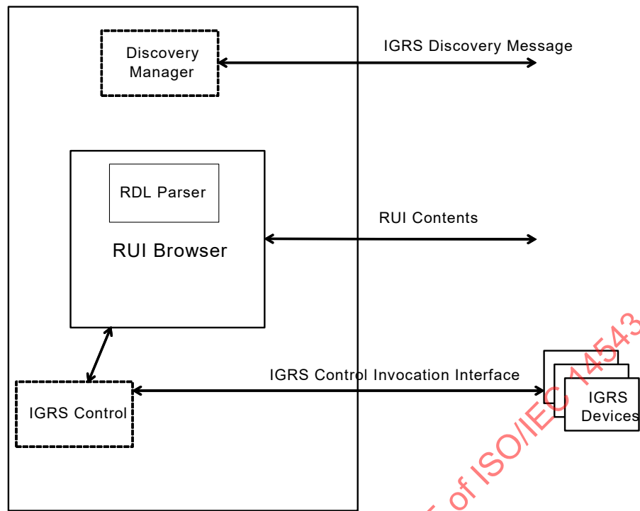
Figure 5 – RUIC architecture
