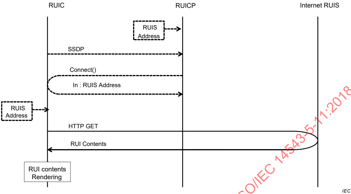
Figure 7 – RUI retrieval from Internet RUIS
