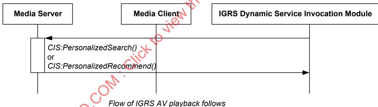
Figure 28 – Flow of content recommendation by online personalization
