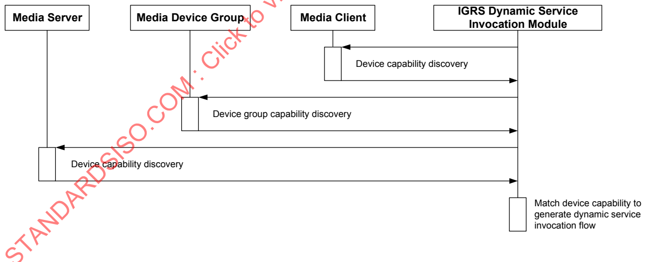
Figure 16 – Interaction flow of dynamic service invocation
