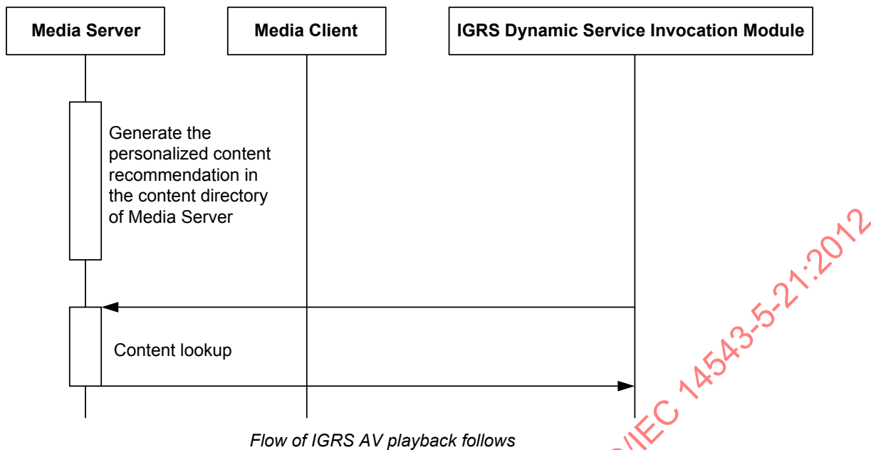
Figure 27 – Flow of content recommendation by offline personalisation
