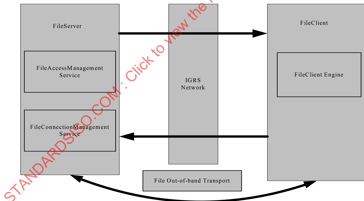
Figure 1 – IGRS file profile interaction model
