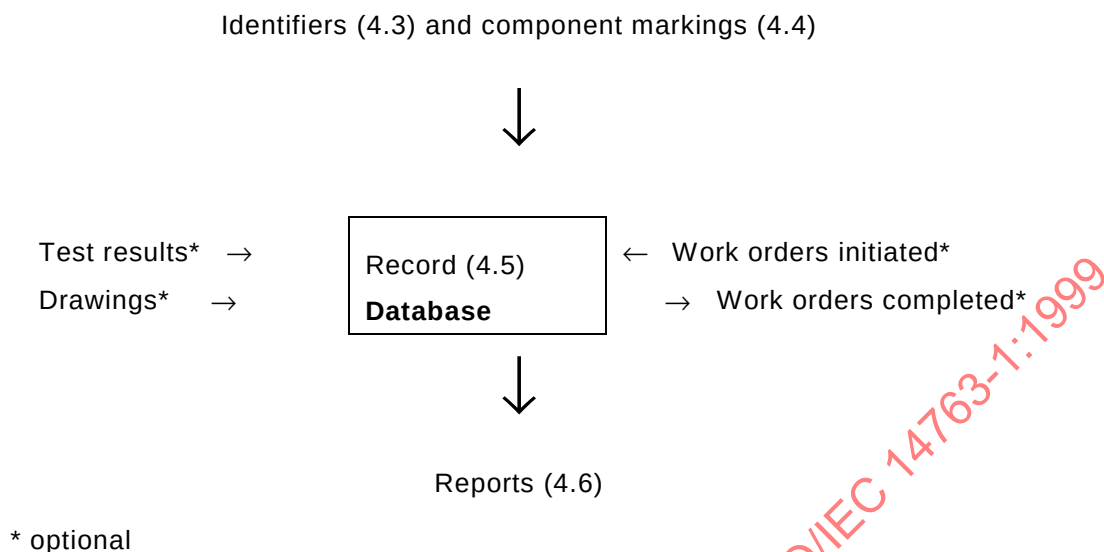
Figure 2 – Basic cabling administration
