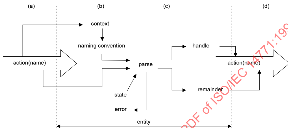
Figure 2 – The general name resolution step
