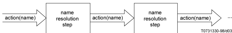
Figure 3 – The name resolution model in cascade
